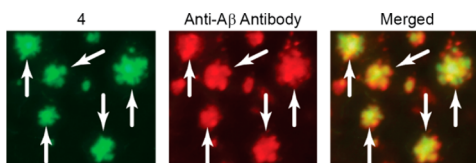
Figure 2. Staining of brain tissue sections (50 \mu\text{m} ) from \text{APP}^{\pm}/\text{PS1}^{\pm} mice using 4 (1 \mu\text{M} ) or immunostained with mouse anti- \text{A}\beta monoclonal antibody (mHJ3.4) conjugated to Alexa Fluor 568 (positive control). Arrows indicate labeling of \text{A}\beta plaques. Similar results were obtained in more than five independent experiments.
