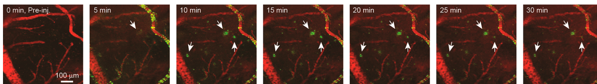
Figure 4. Real time imaging of 4 in brains of \text{APP}^{\pm}/\text{PS1}^{\pm} transgenic mice: Following labeling of blood vessels with dextran–Texas Red, 4 (2 mg/kg) was intravenously injected. A z-stack image series was acquired using an LSM 510META NLO microscope (Carl-Zeiss Inc.).
