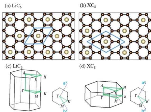
Fig. 2 The planar structures of (a) \text{LiC}_6 and (b) \text{XC}_8 [ X = \text{Na}, \text{K}, \text{Rb} and \text{Cs} ]. The first Brillouin zones of (c) \text{LiC}_6 and (d) \text{XC}_8 [ X = \text{Na}, \text{K}, \text{Rb} and \text{Cs} ].
