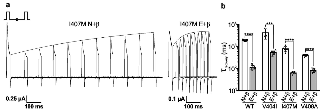
Figure 6. Editing alters the recovery from Kvβ1.1-induced inactivation in V404I, I407M, and V408A channels. Whole-cell K + currents were recorded from oocytes co-expressing the Kvβ1.1 subunit and either a non-edited (N) or edited (E) isoform of the wild-type (WT) or mutant Kv1.1 channel. (a) Representative I407M N and I407M E recovery traces are overlaid to depict the increased rate of recovery from β-inactivation, typical of an E isoform. A two-pulse protocol was used, eliciting a depolarizing pulse to 80 mV followed by a variable interpulse duration at −80 mV before a final depolarizing pulse at 80 mV. Recovery from β-inactivation was plotted as the time for the second pulse to regain the current amplitude of the first pulse. (b) τ values were determined by fitting single exponential curves to the recovery plots (mean ± SEM, n = 3–7 oocytes, ***p ≤ 0.001, ****p ≤ 0.0001).
