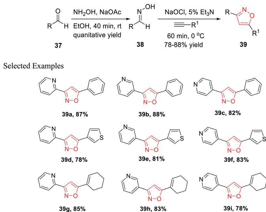
Scheme 9 Synthesis of 3,5-disubstituted isoxazole.
