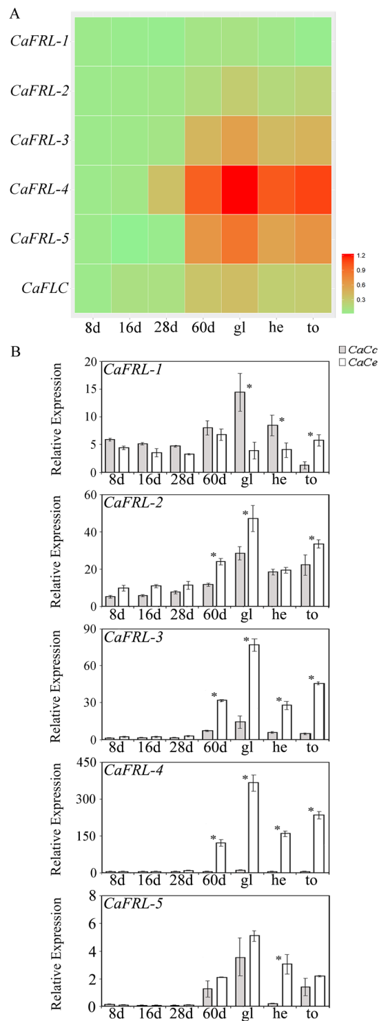
Figure 7. Gene expression analysis of CaFRL genes and CaFLC gene in C. arabica direct somatic embryogenesis ( A ) Heat map visualization of CaFRL expression in DSE at different stages. The sum of relative homeolog expressions was used as numerical input for creating the heat map scale from light green (weakly expressed) to red (strongly expressed). ‘8d’ sample was used as internal calibrator ( B ) Expression profiles of homeologous genes (CaCc and CaCe) of CaFRL family during DSE at different stages: 8 days (8d), 16 days (16d), 28 days (28d), 60 days (60d), globular embryos (gl), heart embryos (he) and torpedo embryos (to). Values of three technical replicates are presented as mean \pm SD (error bars). Transcript abundances were normalized using the expression of UBI (ubiquitin) as reference gene. Asterisks indicate significant differences ( P < 0.05 ) between homeologous genes.
