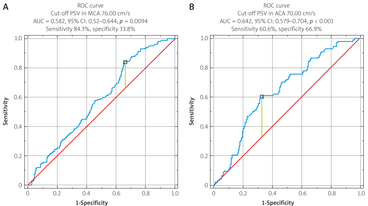
Figure 1. Receiver–operator characteristic (ROC) curves showed no good cut-off values for PSV in MCA or ACA to discriminate increased risk of IS
