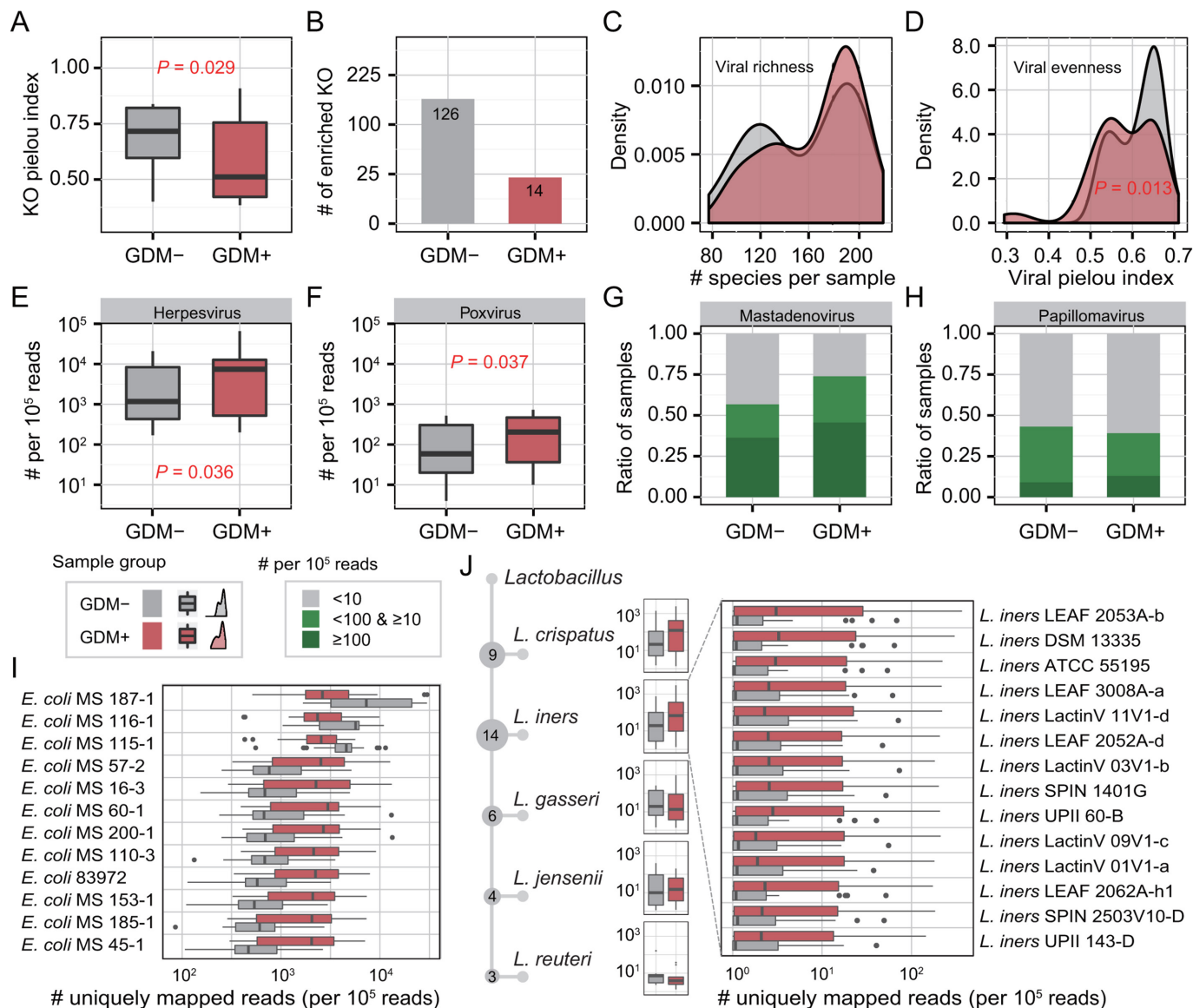
Figure 6 Microbial and functional variation in meconium microbiota associated with gestational diabetes mellitus (GDM). (A) Evenness of the KEGG orthology (KO). (B) The number of enriched KOs. (C, D) Distribution of viral richness and evenness. (E, F) Relative abundance of herpesvirus and poxvirus. Viral abundance in each sample was normalised to 100 000 reads. (G, H) Prevalence of mastadenovirus and papillomavirus in meconium. (I, J) Significant differentiation of Escherichia and Lactobacillus strains between GDM+ and GDM-. Genomes of Escherichia and Lactobacillus strains isolated from the human oral cavity, gut or vagina were downloaded from the Human Microbiome Project (HMP) and were taken as references. Sequencing reads were mapped to these references, and strain abundance in each sample was normalised to 100 000 reads.
