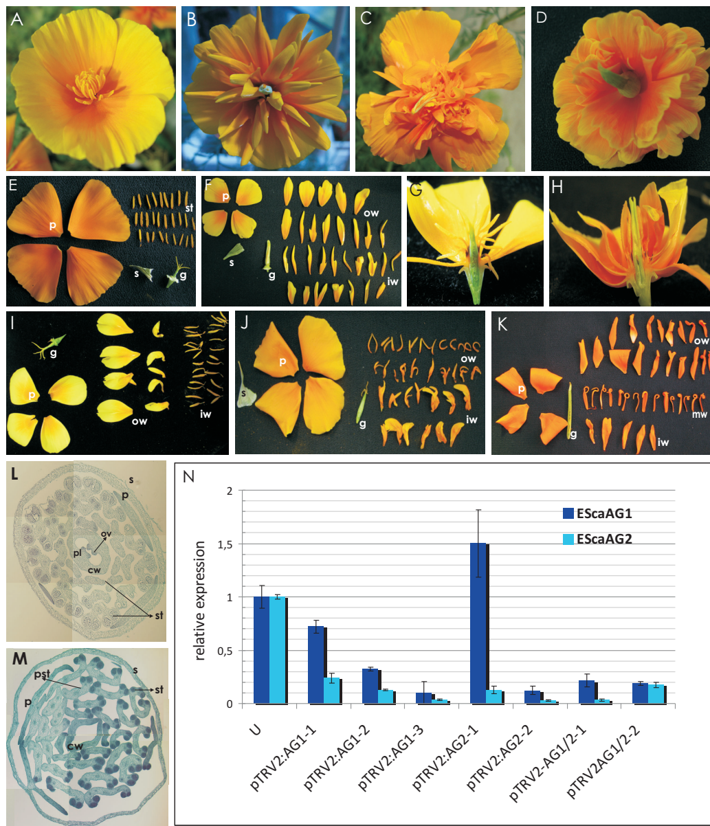
Figure 3 Phenotypes of plants treated with pTRV1 and pTRV2- E ScaAG1, pTRV2- E ScaAG2, or pTRV2- E ScaAG1/2 and expression analysis of the VIGS treated plants. (A) Wild type phenotype of an E. californica flower treated with pTRV2-E. (B) Phenotype of an E ScaAG1 VIGS treated plant showing full homeotic conversions of stamens into petals. (C) Phenotype of an E ScaAG2 VIGS treated plant showing full homeotic conversions of stamens and carpels into petal-like structures. (D) Phenotype of a flower silenced for E ScaAG1/2 showing homeotic conversions of stamens into petals. (E) A mock treated plant with disassembled floral organs. (F) Disassembled flower of a plant treated with pTRV2- E ScaAG1/2 showing homeotic conversions of stamens into petals. The same phenotype was also achieved with plants silenced for E ScaAG1 or E ScaAG2 individually. (G) Transverse hand section of a flower from a mock treated plant. (H) Transverse hand section of a flower from a plant silenced for E ScaAG1/2 showing homeotic conversions of stamens into petals. (I) Disassembled flower of a plant silenced for E ScaAG1 showing partial homeotic conversions of only the outer whorl stamens. (J) Disassembled flower of a plant treated with pTRV2- E ScaAG2 showing that the inner whorl of stamens is converted into petal-like structures. (K) Disassembled flower of a plant treated with pTRV2- E ScaAG1/2 exhibiting homeotic conversions of the innermost and outermost stamens whorls into petals while the middle whorls show mild deviation from wild type stamens while the center whorl stamens remain more stamen-like. (L) Transverse section of a flower of an untreated plant. (M) Transverse section of a flower from an E ScaAG1 VIGS treated plant showing homeotic conversion of stamens into petals, petal-stamen mosaic structures, malformed stamens and a gynoecium lacking tissue differentiation, ovules, and placenta. (N) Real-Time PCR analysis of the first bud of individual E. californica plants treated with VIGS and untreated (U). Plants were treated with pTRV2- E ScaAG1 are abbreviated as VIGS AG1, plants treated with pTRV2- E ScaAG2 as VIGS AG2. Numbers below indicated individual plants and the relative expression level of E ScaAG1 and E ScaAG2 in untreated plants was set to 1. Abbreviations: cw, carpel wall; ov, ovule; p, petal; pl, placenta; se, sepal; pst, petaloid stamens; st, stamen.
