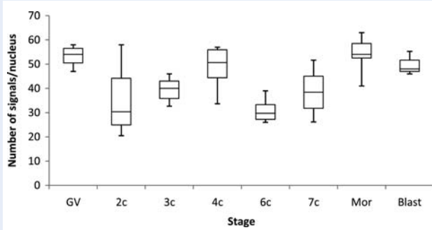
Figure 2 Numbers of telomere signals identified in GV oocytes and embryonic nuclei at different stages of development (2 cell–7-cell, morula, blastocyst). Box plots represent the median and inter-quartile range, with whiskers representing the 5th and 95th percentiles.
