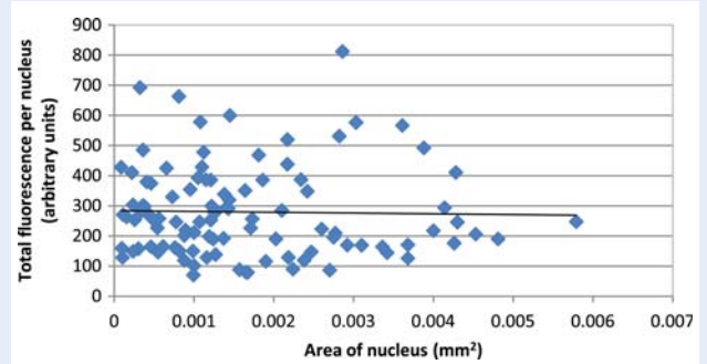
Figure 3 Total telomere-associated fluorescence per nucleus in relation to nuclear area. There was no significant relationship between fluorescence and nuclear area.
