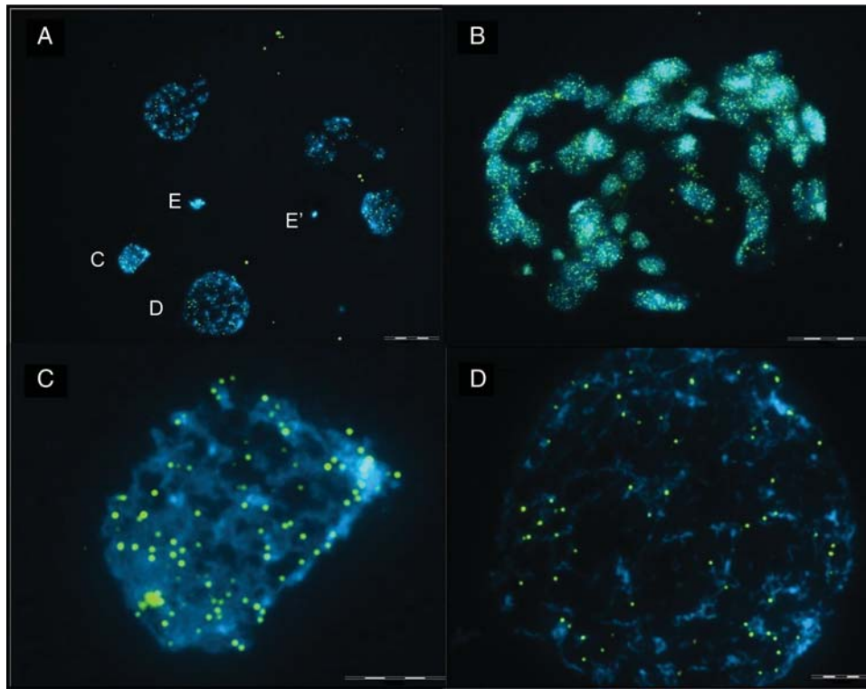
Figure 1 Telomeres in human embryos. Telomeres were stained using a FITC-labelled pan-telomeric probe (green). All nuclei were counterstained with DAPI (blue). (A) 6-cell embryo resulting in five nuclei with two polar bodies, E and E' (scale bar = 44 \mu\text{m} ). Two of the nuclei ( C and D , scale bar = 8.5 \mu\text{m} ) are also shown under higher magnification (scale bar = 4 \mu\text{m} ). (B) The telomeres in a fixed blastocyst (scale bar = 55 \mu\text{m} ).
