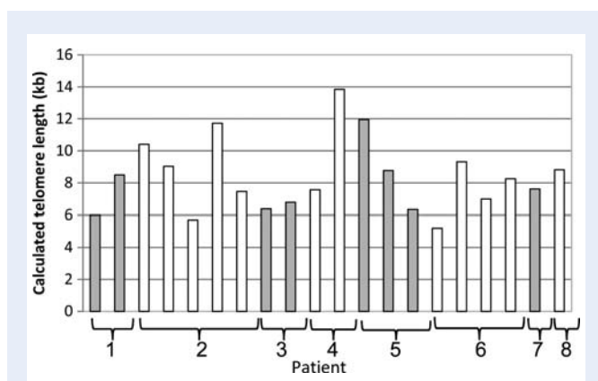
Figure 7 Average calculated telomere lengths of individual human embryos originating from different patients. The embryos are arranged into eight groups according to the couple from whom they originated. Couple 8 donated the morula, although the other embryos are from 2-cell to 8-cell stage.
