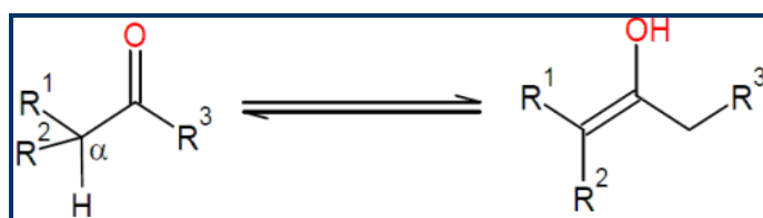
Figure 1: Keto and Enol forms of nucleotides
