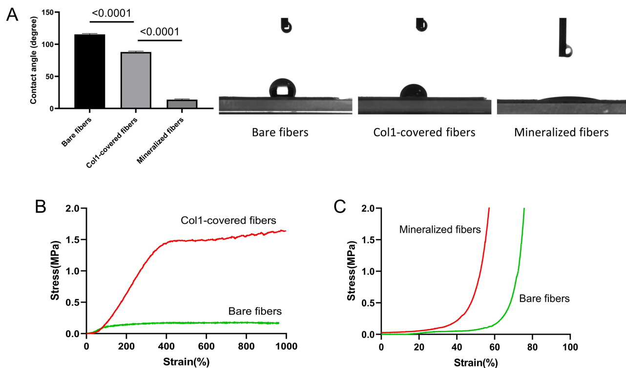
Figure 4 (A) Water contact angles of unmodified and modified scaffolds (n=3). (B) Tensile tests of scaffolds coated with Col1 versus unmodified scaffolds. (C) Compression tests of scaffolds coated with HA versus unmodified scaffolds.
