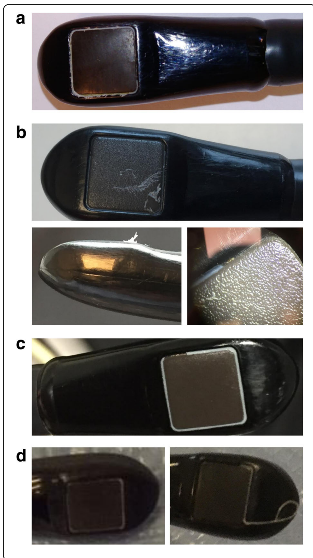
Fig. 2 Common pattern of damage of transesophageal echocardiography probes. All affected probes were of the same type (X7-2t transducer; Philips, Amsterdam, The Netherlands). a TEE probe of operating room A, beginning of July 2017. The silicone bead around the transducer lens was peeling off and was almost completely missing at one side (the side facing the shaft of the probe). This defect was accompanied by the complete absence of the protective polyethylene film that normally should cover the transducer lens. Shredded polyethylene film fragments can be seen along the remaining parts of the silicone seal. Orange discoloration of some ragged polyethylene film fragments and brown-yellow deposits in the area of the torn-off silicone bead cannot be seen on this picture, but were observed when the TEE probe was examined under a stereoscopic microscope (no pictures available) and were indicative of the presence of cellular debris and organic material. b TEE probe of CSICU, mid July 2017. A large part of the silicone bead was missing and the polyethylene film had partially come loose and was ruptured (top). The side view of the probe tip illustrates the detachment and rupture of the polyethylene film (bottom left). Yellow deposits can be seen in the area of the missing silicone bead (bottom right). c TEE probe of CICU, end of January 2018. A section of the silicone bead was missing. d TEE probe of the cardiology polyclinic, February 2018. The TEE probe appeared intact at the beginning of February 2018 (left), but a new inspection 3 weeks later revealed that a large part of the silicone bead had suddenly come off (right). Abbreviations: CICU cardiac intensive care unit, CSICU cardiac surgery intensive care unit, TEE transesophageal echocardiography
