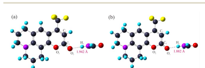
Fig. 3 Optimized geometric structures for the C540A-FA complex in S_0 (a) and S_1 (b) at the B3LYP/TZVP/IEF-PCM (FA) level.
