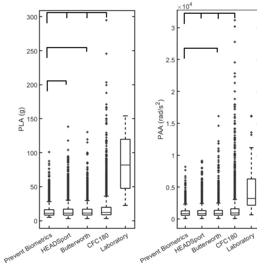
Figure 4 Peak linear acceleration (PLA) and peak angular acceleration (PAA) based on the Prevent Biometrics processed output, HEADSport filter method, Butterworth-200Hz and CFC180 filter approach. Boxplots indicate the median (box midline), IQR (box) and most extreme data points (whiskers) not considered outliers (crosses). Outliers are values greater than 1.5 times the IQR from top of the box. Horizontal lines above boxplots indicate statistical significance ( p < 0.05 ). Laboratory impacts were not included in the mixed linear effects models. Boxplots with outliers removed can be seen in online supplemental material B.
