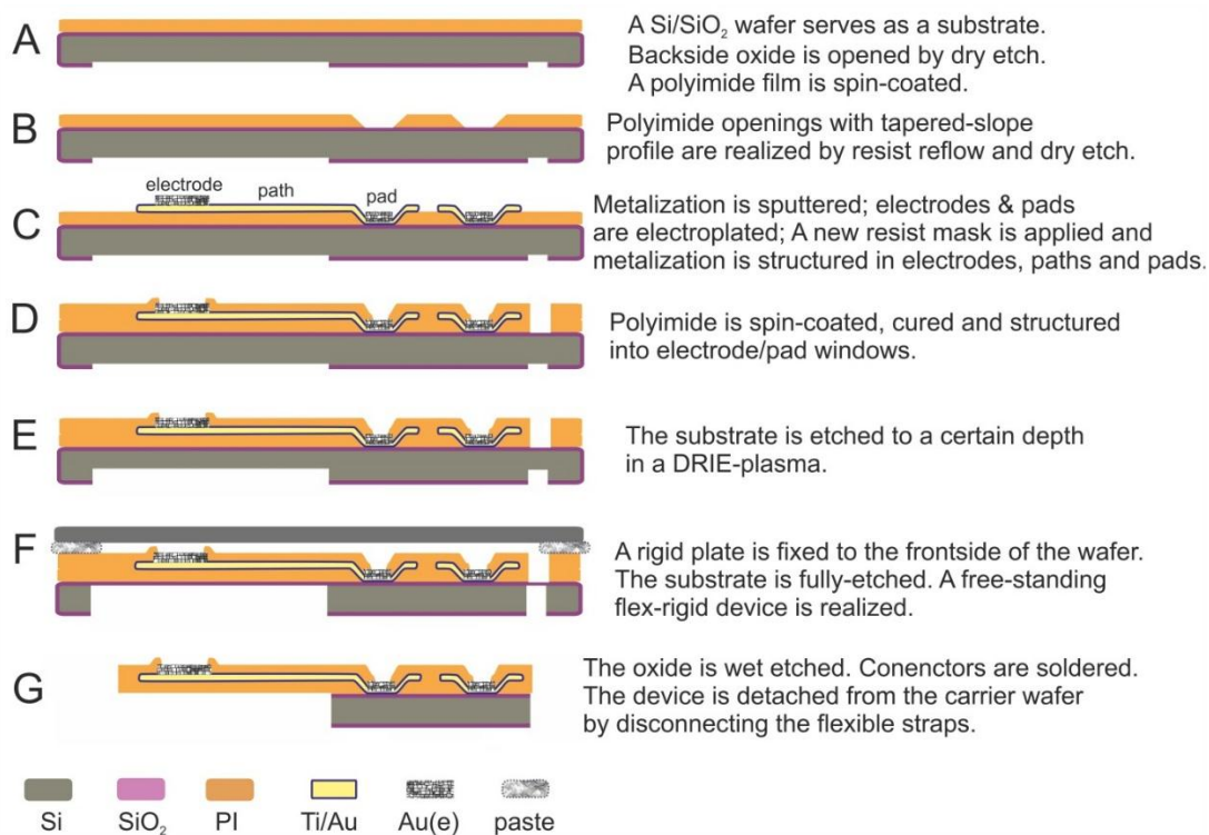
Figure 3. Microfabrication flow.
