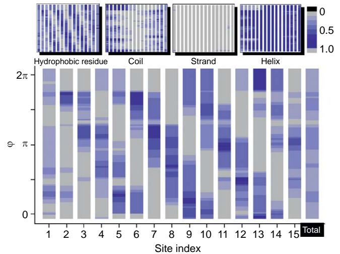
Fig. 3. Buried residues of a donut ring for K > 140 as a function of \varphi . Samples in each pie slice are matched site by site. At each site, the probability of a buried residue is shown by different brightness. The insert shows the distribution of hydrophobic residues and secondary structures obtained by the same method.
