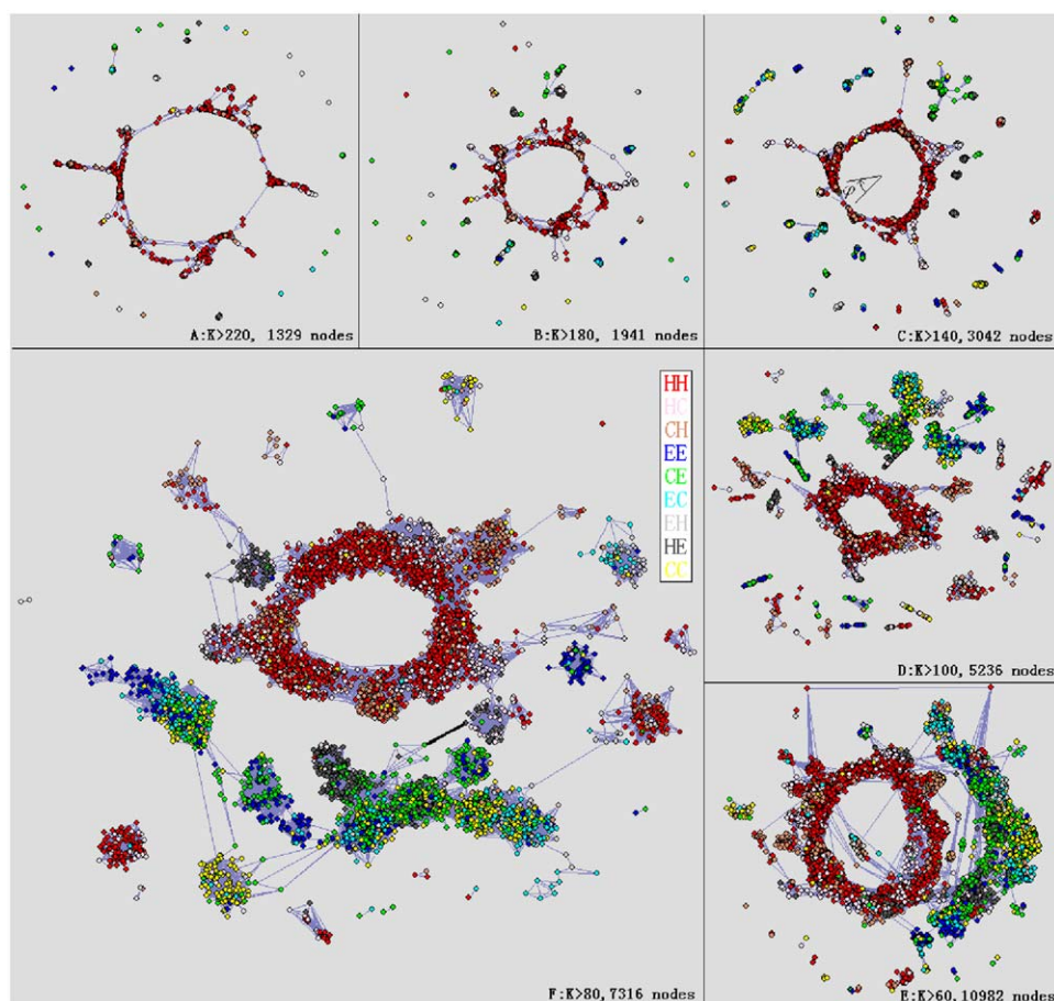
Fig. 2. Donut-shaped fingerprint of the polypeptide relationship network. Nodes with a connection number K greater than 60 are plotted. Orphans in these subnetworks are omitted. Tightly related nodes are bunched up by PAJEK. The donut is rich in HH + HC + CH samples. The arc in E is rich in EE + EC + CE samples. A connected strand-arc is evident in F. In F, there is only one edge (colored in black) that connects the helix-donut to strand-arc.
