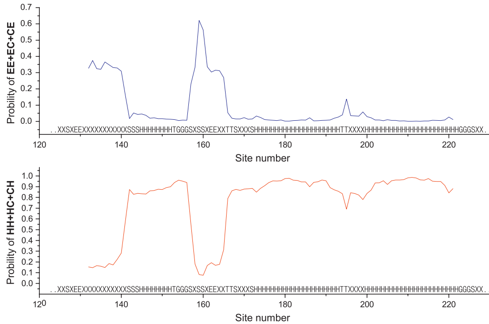
Fig. 4. Frequency of two types of nodes connected to agents of the query segments of human prion protein 1QM2.
