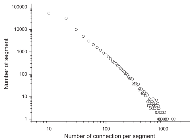
Fig. 1. Node population as a function of connectivity.
