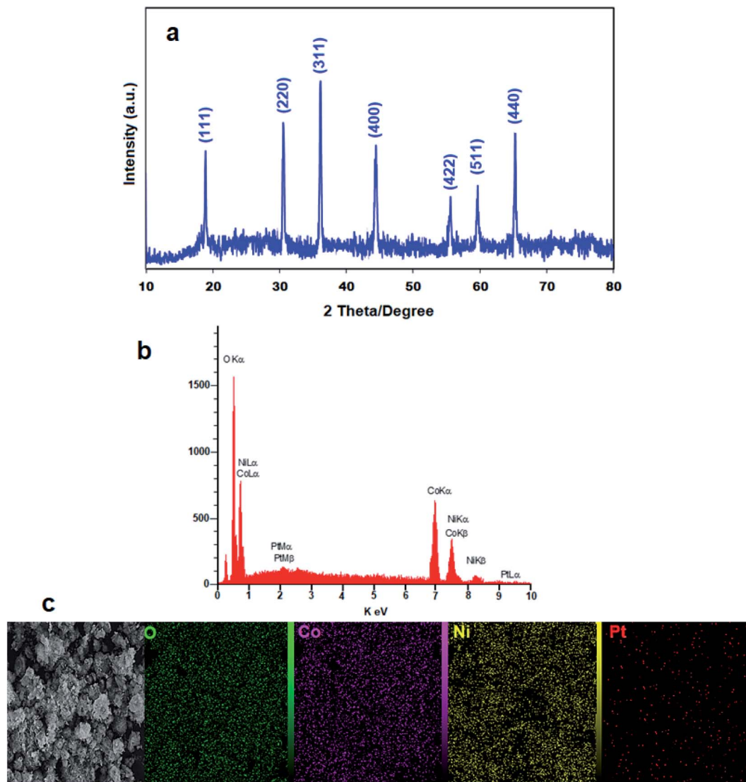
Fig. 1 (a) XRD pattern, (b) EDX spectrum and (c) elemental mapping for flower-like Pt/NiCo 2 O 4 nanocomposite.
