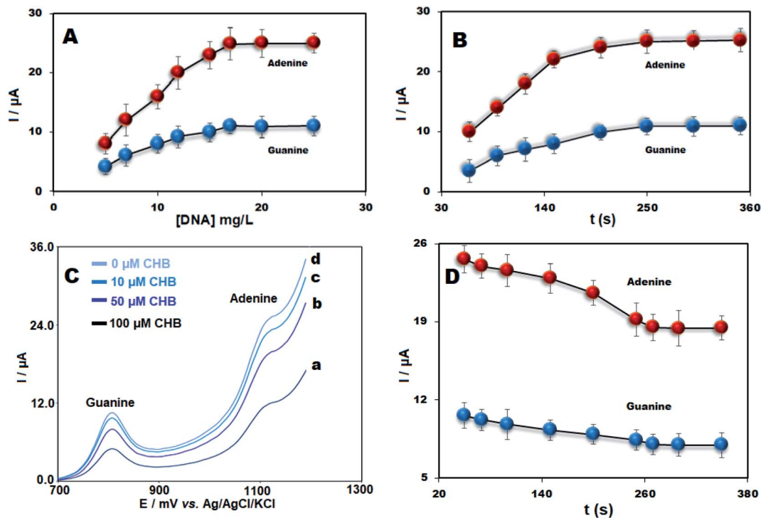
Fig. 4 (A) The plot of oxidation signal of adenine and guanine vs. diverse ds-DNA concentrations (5–25 \text{mg L}^{-1} ) and (B) various accumulation time. (C) DPV for ds-DNA/PPy/FL-Pt/NiCo 2 O 4 /PGE in the presence of (a) 0, (b) 10, (c) 50 and (d) 100 \mu\text{M} CHB and (D) The incubation time effect of 50.0 \mu\text{M} CHB on the response of ds-DNA/PPy/FL-Pt/NiCo 2 O 4 /PGE ( n = 3 ).
