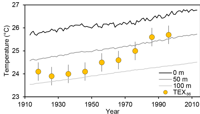
Fig 6. Long-term \text{TEX}_{86} temperature data compared to model estimates. Each large orange circular dot is a raw \text{TEX}_{86} surface temperature measurement. Each \text{TEX}_{86} measurement represents the annual mean surface temperature at the location of the \text{TEX}_{86} core site \pm 0.4^\circ\text{C} (95% confidence interval). The three lines are the modeled annual surface temperature at the location of the \text{TEX}_{86} core site at three different depths (0, 50, 100 m). There is a strong disagreement between \text{TEX}_{86} and modeled in situ temperatures, especially early in the time series. Deviations between the \text{TEX}_{86} temperature measurements and the modeled surface temperature may reflect model error, error in the \text{TEX}_{86} calibration procedure, or long-term shifts in the depth range of Thaumarchaeota (the microbes whose biomolecules are involved with generating the \text{TEX}_{86} proxy).
