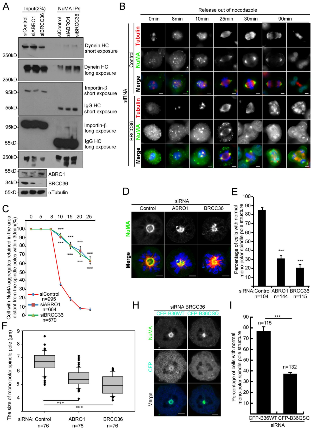
Figure 8. BRISC modulates the function of NuMA in spindle pole assembly. (A) Depletion of BRISC regulates the interaction of NuMA with dynein and importin- \beta . HeLa cells transfected with control, ABRO1, or BRCC36 siRNA for 72 h were collected, and protein samples were analyzed by Western blotting with the indicated antibodies. (B) Depletion of BRISC decreased the incorporation of NuMA into the spindle poles during mitosis. HeLa cells transfected with control or BRCC36 siRNA were treated as described in MT regrowth assay in Materials and methods, and immunostained for \alpha -tubulin (red) and NuMA (green). (C) Quantitative analysis of cells in which NuMA did not completely incorporate into the spindle poles within 25 min after NOC release. Mean \pm SD of three independent experiments. ***, P < 0.001 ; Student's t test. (D) Representative images of the K-fiber minus ends distribution of NuMA. Control,
