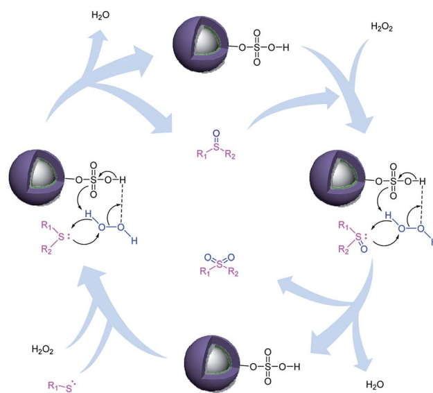
Scheme 4 Proposed mechanism for the oxidation of sulfides to sulfoxides or sulfones in the presence of Fe 3 O 4 @BNPs@SiO 2 -SO 3 H with H 2 O 2 as a green oxidant.
