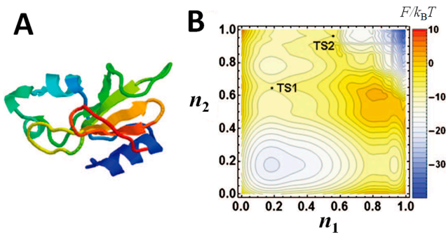
Figure 4 Application of the WSME model to barnase. A) Native conformation of barnase from Bacillus amyloliquefaciens (PDB code: 1a2p). B) Two-dimensional free-energy landscape, F(n_1, n_2) , calculated with the WSME model, where n_1 is the order parameter of folding of the N-terminal half, and n_2 is the one of the C-terminal half. Contour is drawn in every 2k_B T . F(n_1, n_2) has four basins; basin of unfolded state ( n_1 \approx 0.2, n_2 \approx 0.2 ), basin of native state ( n_1 \approx 1.0, n_2 \approx 1.0 ), and two basins of intermediate states, I_1 ( n_1 \approx 0.2, n_2 \approx 0.8 ) and I_2 ( n_1 \approx 0.9, n_2 \approx 0.2 ). Saddles around the basin I_1 are much lower in free energy than those around I_2 are; therefore, a pathway through I_1 is a dominant pathway, and I_1 is a dominant intermediate. I_2 could be detected as an off-pathway intermediate. Along the dominant pathway, there are two transition states, TS1 and TS2. Modified from Figure 14 of [20] with permission.
