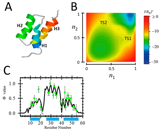
Figure 3 Application of the WSME model to the B domain of Staphylococcal protein A (BdpA). A) Native conformation of BdpA (Protein Data Bank (PDB) code: 1bdd). B) Two-dimensional free-energy landscape, F(n_1, n_2) , calculated with the WSME model, where n_1 is the folding order parameter of the N-terminal half, and n_2 is the one of the C-terminal half. A contour is drawn every 0.5k_B T . F(n_1, n_2) has two basins: the unfolded state basin ( n_1 \approx 0.3, n_2 \approx 0.3 ) and the basin of the native state ( n_1 \approx 1.0, n_2 \approx 1.0 ). Two transition states, TS1 and TS2, are shown; there are two dominant pathways of folding, which proceed through TS1 and TS2. C) Comparison of the calculated and observed \Phi -values. The calculated values are shown with a line and the observed values [37] are green squares shown with error bars. Bars on the bottom represent the positions of \alpha helices. Modified from Figures 1, 3, and 5 of [15].
