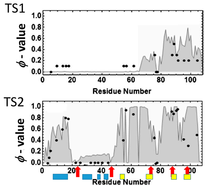
Figure 5 Calculated and observed \Phi -values at the two transition states, TS1 and TS2, of barnase. Lines shaded with gray correspond to the calculated \Phi -values with the WSME model. Dots are the experimentally observed values [39,40]. Red arrows are boundaries of modules defined by the pattern of atomic contacts in the native conformation [44,45]. Bars shown on the bottom represent secondary structure elements, helices (blue) and strands (yellow). Modified from Figure. 15 of [20] with permission.
