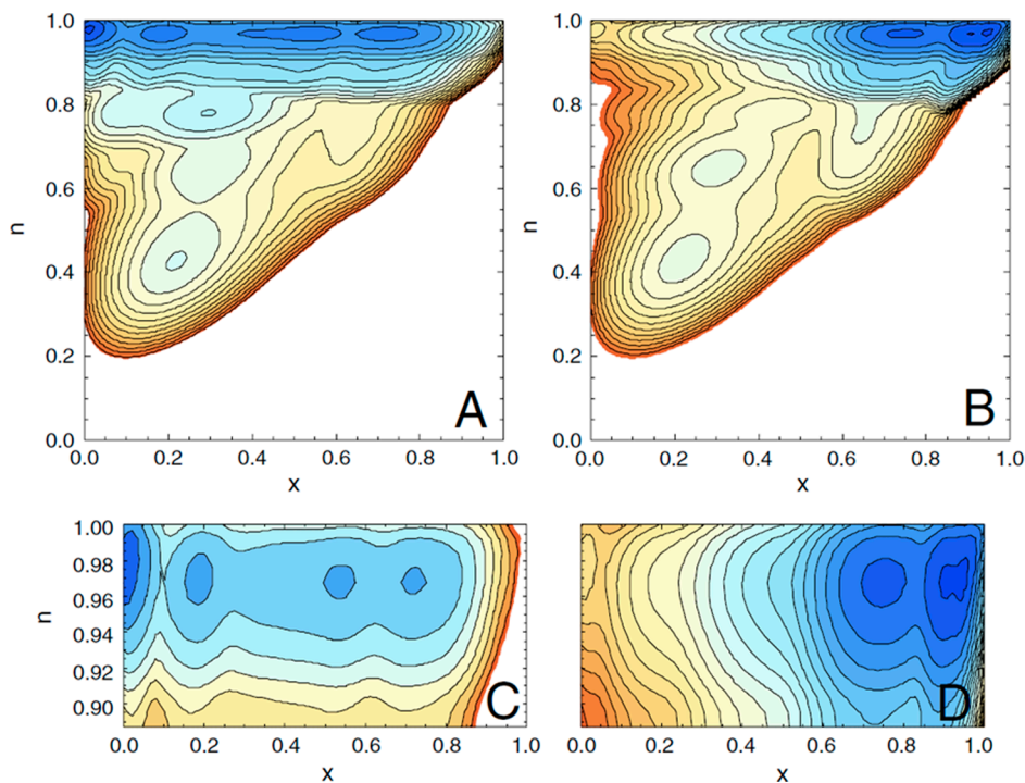
Figure 10 Free-energy landscape F_\alpha(x, n) of allosteric transition of NtrC calculated with the aWSME model. x is the order parameter of folding transition and n is the order parameter of allostery transition. (x, n) = (0, 1) is the I conformation, (1, 1) is the A conformation, and (0, 0) is the completely disordered state. A) F_{\text{dephos}}(x, n) in the dephosphorylated state and B) F_{\text{phos}}(x, n) in the phosphorylated state. C) and D) are closeups of A) and B), respectively, at n \approx 1 . Contour is drawn for every 2k_B T . Reproduced from [31].
