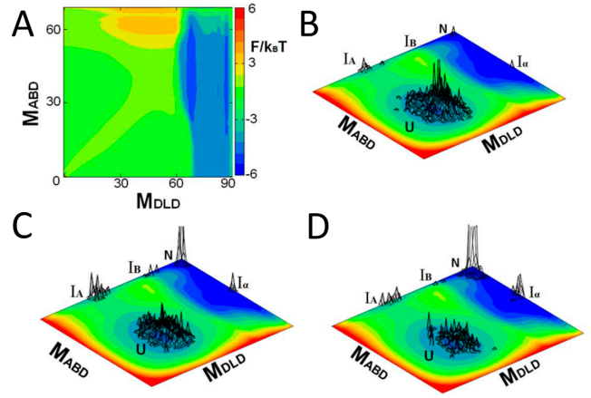
Figure 8 Free-energy landscape and folding kinetics of the circular permuted of DHFR calculated by the eWSME model. A) Difference in the free-energy landscape between the wild type and the circular permuted of DHFR. B–D) Evolution of the population of 200 molecules simulated with the Monte Carlo calculation at B) 3.3 \times 10^5 t_0 , C) 1.6 \times 10^6 t_0 , and D) 3.0 \times 10^6 t_0 , where t_0 is a unit of time in simulation. Reproduced from [23].
