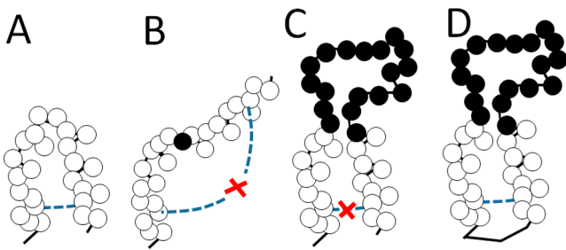
Figure 1 The native interaction in the WSME model. Residues in the native-like configuration are shown with white circles, and residues in non-native configurations are shown with filled circles. A) The native interaction (a blue dashed line) between the residues within a contiguous native-like segment is taken into account in the WSME model. B) The interaction becomes ineffective when an intervening residue is in the non-native configuration. C) If the linker chain connecting two native-like segments is long enough, a number of residues with random configurations can compensate each other to allow two segments to reach the positions where native interactions are effective. This type of interaction, however, is not taken into account in the WSME model. D) Interactions as in C can be suitably calculated with the WSME Hamiltonian if we consider that the N- and C-termini are connected by a virtual link, as explained in the section “The WSME Model for Multi-domain Proteins”.
