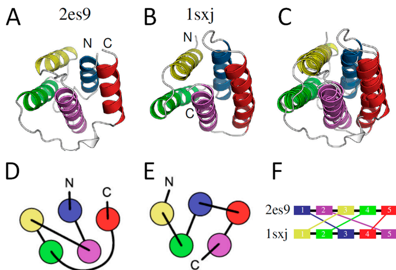
Figure 12 An example of a non-sequential structure alignment. A) Structure of Q8ZRJ2 (PDB code: 2es9), B) structure of the eukaryotic clamp loader (PDB code: 1sxj), and C) the superimposition of Q8ZRJ2 and the eukaryotic clamp loader obtained by the non-sequential alignment program MICAN [70]. In A–C, the structurally equivalent regions are drawn with the same color. It can be clearly seen that all helices are well superimposed if both the chain direction and the connectivity are ignored. D and E are two-dimensional diagrams of protein topology of Q8ZRJ2 (A) and eukaryotic clamp loader (B), respectively. F) Correspondence relation of helices obtained by MICAN. Reproduced from [73] with permission.
