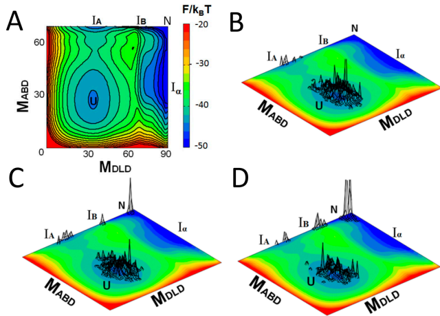
Figure 7 Free-energy landscape and kinetics of DHFR folding calculated by the eWSME model. A) Free-energy landscape of DHFR folding represented in the two-dimensional space of M_{DLD} and M_{ABD} . The landscape has basins corresponding to the unfolded state U, the native state N, and the intermediates, I_A , I_B , and I_\alpha . B–D) Evolution of the population of 200 molecules simulated with the Monte Carlo calculation at B) 3.3 \times 10^5 t_0 , C) 1.6 \times 10^6 t_0 , and D) 3.0 \times 10^6 t_0 , where t_0 is a unit of time in simulation. Reproduced from [23].
