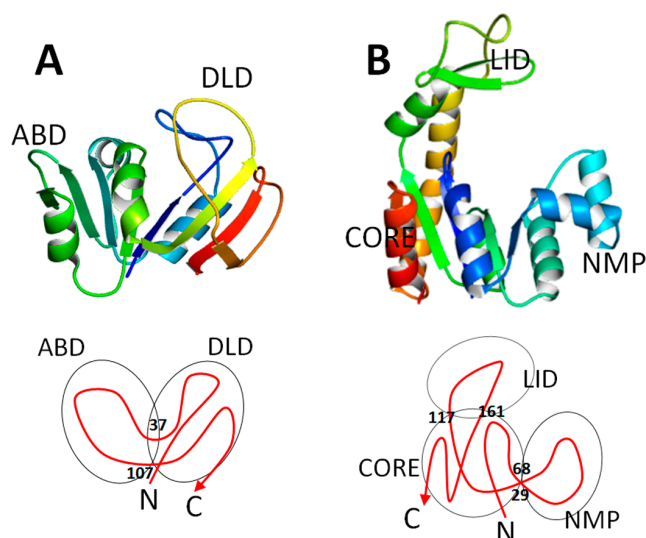
Figure 6 Examples of multi-domain proteins with non-trivial topology. A) Dihydrofolate reductase (DHFR) (PDB code: 1rx1) has two domains, DLD and ABD. B) Adenylate kinase (AdK) (PDB code: 4ake) has three domains, CORE, NMP, and LID. Topological connectivity of the chain is illustrated at the bottom.
