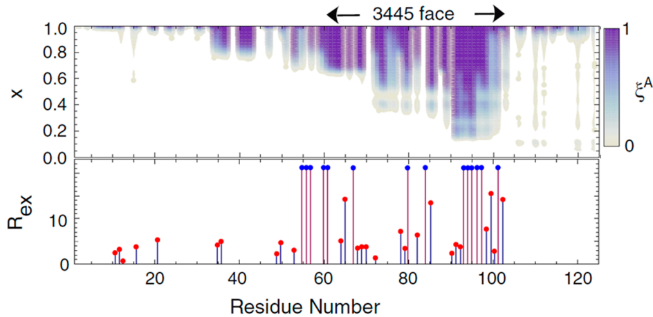
Figure 11 Pre-existing structural fluctuation of NtrC. (Top) The parameter \xi^A showing the extent of the A-like structure development in the dephosphorylated state. \xi^A calculated with the aWSME model under the constraint of each fixed x and n=1 is plotted in gray scale. Even in conformations near the I conformation with small x , the A-like structure appears as a fluctuation around the 3445 face. (Bottom) R_{ex} observed in the relaxation measurement of NMR in the dephosphorylated state [61] are shown with red dots. R_{ex} is larger than a threshold for the blue dots [61]. Reproduced from [31].
