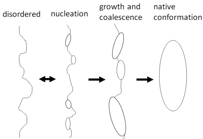
Figure 2 The hierarchical process of protein folding. Folding starts with the creation of contiguous segments with a native-like configuration. After nucleation, folding proceeds as those segments grow and coalesce into larger regions to reach native conformation.
