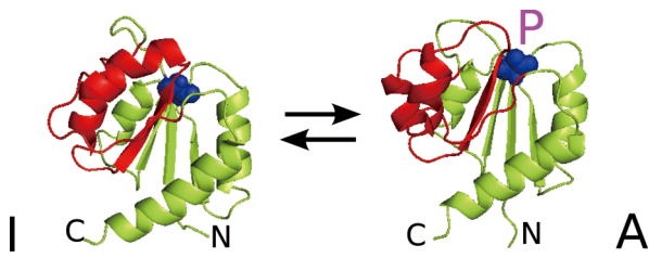
Figure 9 Allosteric transition of NtrC. Upon phosphorylation of Asp54, the NtrC structure switches from a state around the inactive (I) conformation (PDB code: 1dc7) to another state around the active (A) conformation (PDB code: 1dc8). Asp54 is shown with blue colored spheres. “3445 face” (the region comprises helices and strands, \alpha 3 , \beta 4 , \alpha 4 , and \beta 5 ) is colored red. Reproduced from [31].
