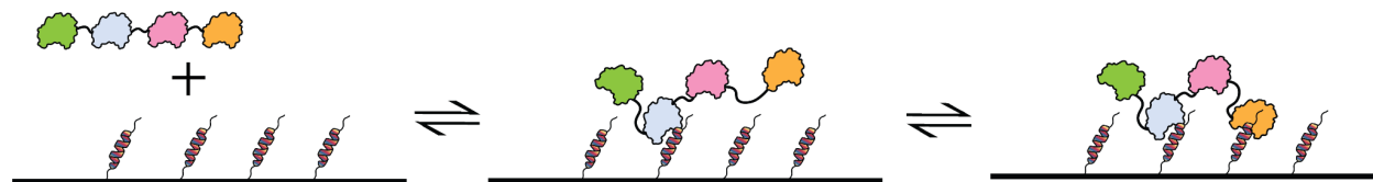
Supplementary Note Figure 1 | Avid binding between a multi-domain co-A and multi-site AD.
