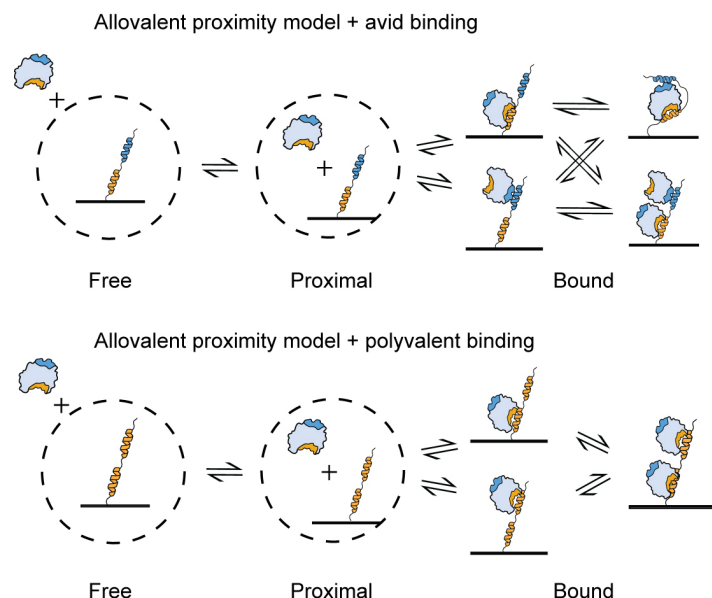
Supplementary Note Figure 3 | Allovalent binding model representing three states: free, proximal, and bound for both avid (top) and polyvalent binding (bottom).
