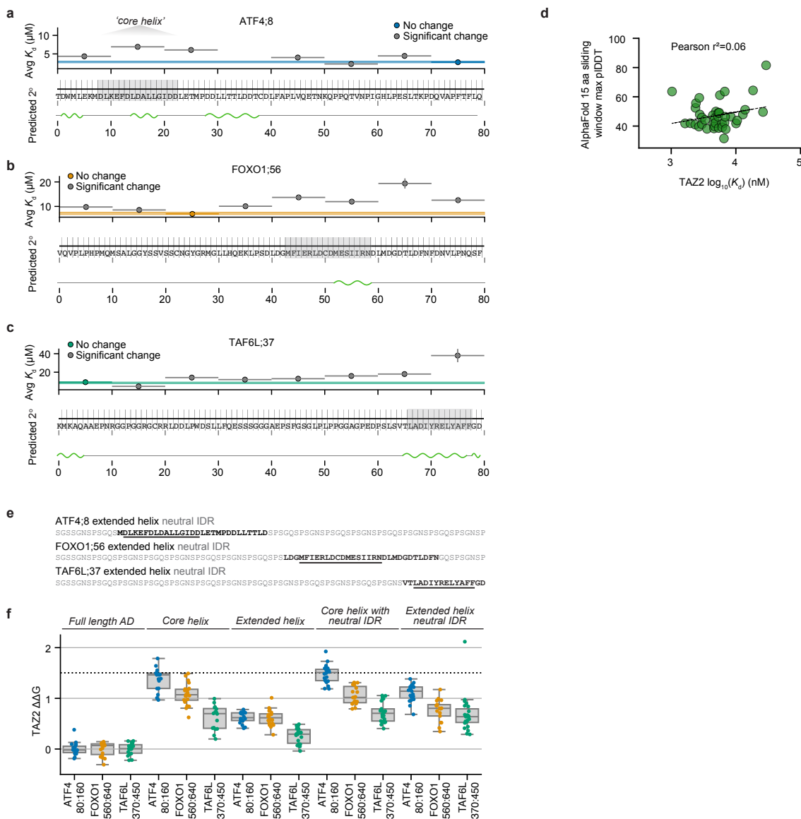
Extended Data Figure 4 | Related to Figure 2 a , STAMMPING-measured affinities ( K_d s) (top), sequence (middle) and AlphaFold-predicted secondary structure (bottom, green regions denote alpha helices, prediction from whole protein sequence) for constructs containing 10 amino acid deletions (deletion locations denoted by horizontal lines) within the TAZ2-binding AD tile ATF4;8. Blue line indicates measured affinity for the wild-type AD tile; vertical height of the line denotes the average standard error of fits across replicates. Deletions are colored by statistical significance (one-sided z-test): deletions with p -values <0.05 (gray) are significantly different from WT, while the rest are not (colors). Grey box highlights the 'core helix'. b , Results as shown in a for the FOXO1;56 AD tile. c , Results as shown in a for the TAF6L;37 AD tile. d , Scatter plot showing AlphaFold-Multimer-predicted confidence scores vs. STAMMPING affinities for 54 TAZ2-binding ADs. e , Rationally designed neutral IDR sequences that were tested in panel f (last column). Underline indicates 'core helix' residues. f , Boxplots show median \Delta\Delta G and interquartile range for TAZ2 binding to different rationally designed mutants of ATF4;8, FOXO1;56, and TAF6L;37. \Delta\Delta G s were calculated in reference to each wild-type AD's K_d . Dashed line is the noise floor for this experiment, defined as the average relative affinity for negative control meGFP binding to TAZ2.
