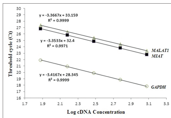
Figure 3: Standard curve for MALAT1 , MIAT and GAPDH . Standard curve is generated by plotting CT values against the logarithm of the cDNA concentration. Pearson's correlation coefficients (square values – R^2 ) is shown. Standard curve of MALAT1 , slope= -3.36 , y-intercept = 33.15, R^2 = 0.999 . Standard curve of MIAT , slope= -3.35 , y-intercept = 32.4, R^2 = 0.997 . Standard curve of GAPDH , slope= -3.41 , y-intercept = 28.34, R^2 = 0.999
