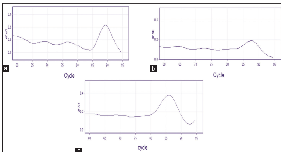
Figure 2: The melting analysis of the Real-time PCR assays. Melting peaks at (a) 88.7°C for MALAT1 gene, (b) 88.2°C for MIAT gene and (c) 85.8°C for GAPDH gene indicate the formation of the tree specific products with different T_m temperatures
