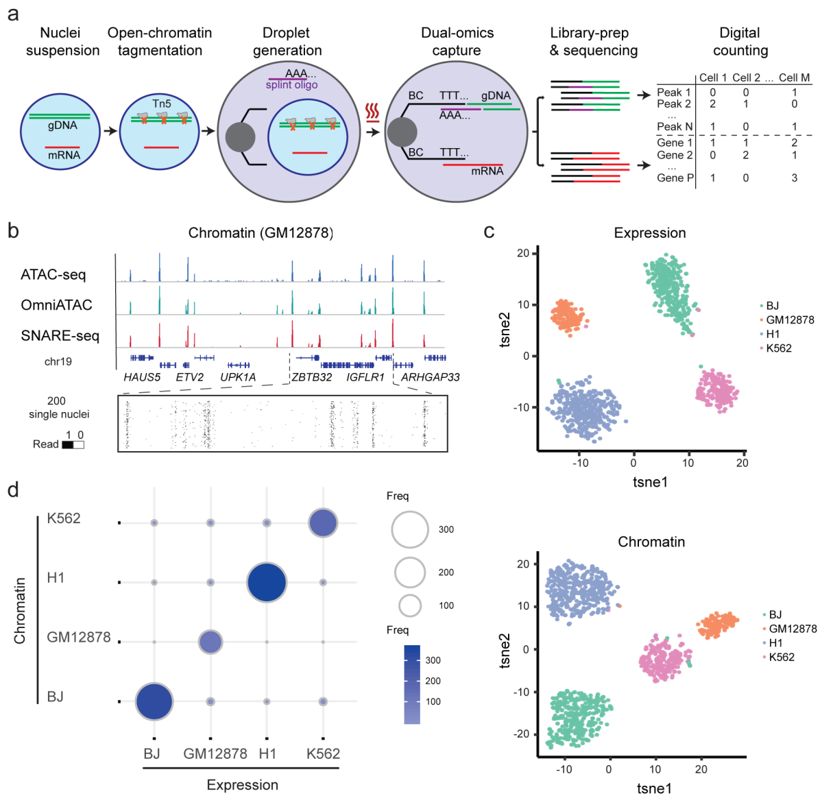
Figure 1. Linked single-nucleus transcriptome and chromatin accessibility sequencing of human cell mixtures. a , Workflow of SNARE-seq. Key steps are outlined in the main text. b , Aggregate single-nucleus chromatin accessibility profiles recaptured published profiles of ATAC-seq and Omni-ATAC in GM12878 cells. c , t-SNE visualization of SNARE-seq paired gene expression (upper panel) and chromatin accessibility (lower panel, n=1,047 ) data from BJ, GM12878, H1 and K562 cell mixture. Cellular identities are colored based on independent clustering results with either expression or chromatin data. d , Inter-assay identity agreement reveals consistent linked transcriptome and chromatin accessibility profiles of SNARE-seq data. The size and color depth of each circle represents the number of cellular barcodes that were identified by the different assays.
