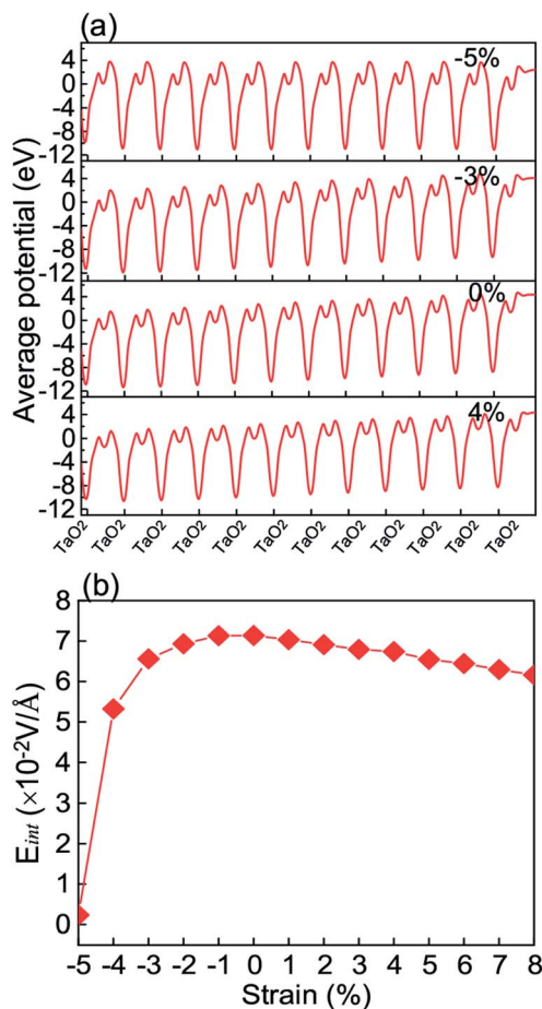
Fig. 3 (a) The monolayer-resolved plane-averaged electrostatic potentials of the KTO slab for strain \varepsilon_s = -5\% , -3\% , 0\% , and 4\% , respectively. (b) The internal electric field ( E_{\text{int}} ) as a function of the strain \varepsilon_s .
