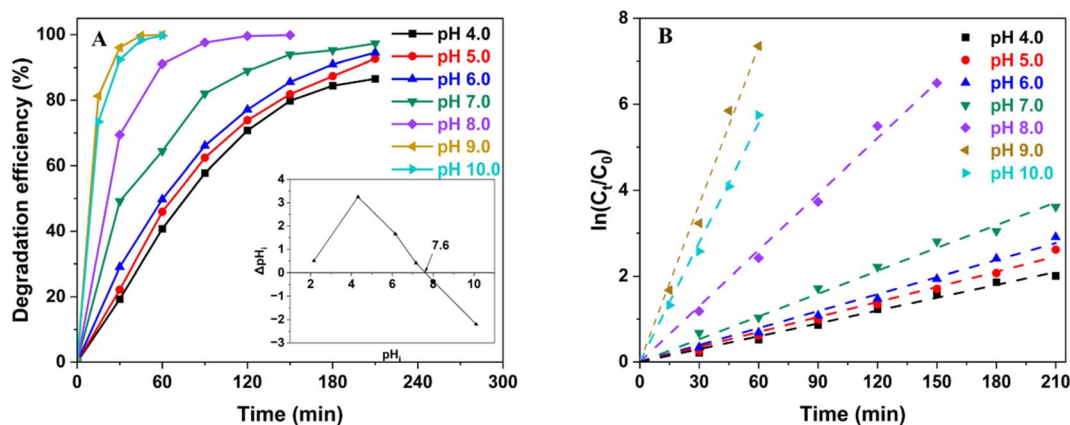
Fig. 9 Influence of pH on (A) RhB photodegradation efficiency (inset figure: determination of the pH_z of ZTC) and (B) degradation kinetics.
