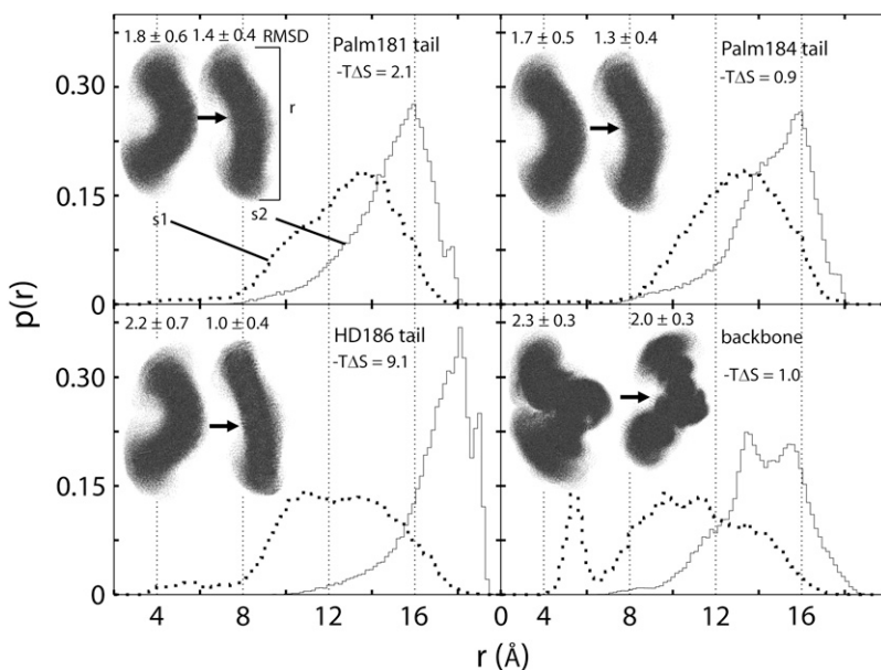
FIGURE 3 Probability ( p(r) ) distribution plots in s1 (dotted line) and s2 (solid line) of the end-to-end distances between the first and last carbon atoms of ANCH lipid tails (Palm181 (top left), Palm184 (top right), HD186 (bottom left)) and between the \text{C}\alpha atoms of residues 180 and 186 (backbone, bottom right). The corresponding structures are shown as dots (inset: s1 \rightarrow s2 ) representing 1-ps-separated snapshots superimposed onto the first frame. The respective average RMSDs are depicted at the top of each structural model. Note that -T\Delta S represents the free energy difference (due to configurational entropy) between states s1 and s2 .
