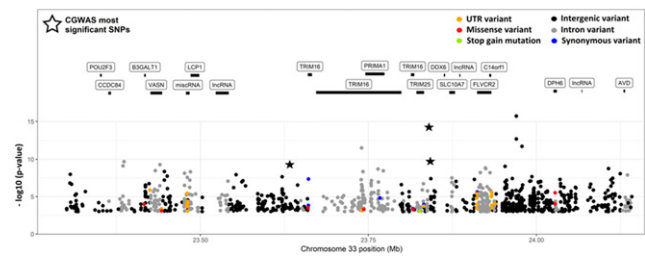
Figure 4 Annotation of the QTL region on chromosome 33 (linkage group 44) including identification of putative genes in the region, functional annotation of SNPs.
