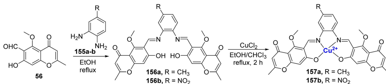
Scheme 48 Synthesis of ligands 156a–b and Cu(II)-metal complexes 157a–b .
