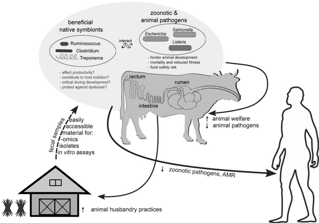
FIG. 1. Overview of the FI vision and goals, the relevant research areas, and how successful implementation could improve animal health and nutrition and reduce the zoonotic and AMR exposure risk to humans. Black arrows show benefits. On top (highlighted with a light blue background), the two main microbial groups of interest (separated based on whether they are beneficial mutualists or animal/zoonotic pathogens) and their implications to potential human exposure and animal husbandry practices are presented. AMR, antimicrobial resistance; FI, Fecobiome Initiative.
