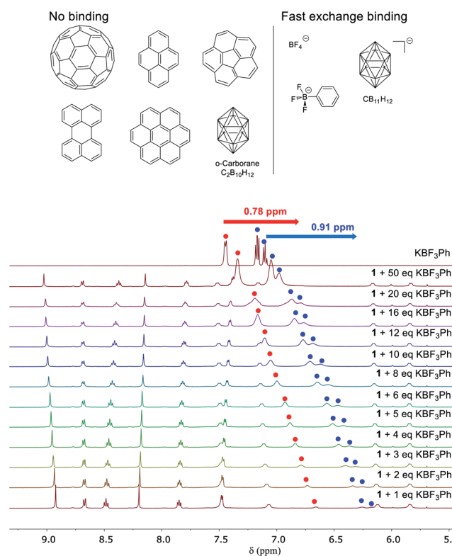
Fig. 3 Top, neutral aromatic non-guests and anionic guests for cage 1 ; bottom, a stacked plot of the ^1\text{H} NMR titration (500 MHz, 298 K) of \text{KBF}_3\text{Ph} into a solution of 1 (0.17 mM) in \text{CD}_3\text{CN} . The signals from the guest ( \text{KBF}_3\text{Ph} ) have been labelled with red and blue dots, and the others belong to cage 1 .
