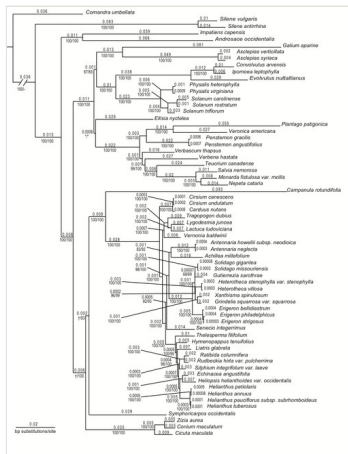
Figure 1. Maximum likelihood (ML) tree (-ln L=46268.63) inferred from the concatenation of 76 plastid, six mitochondrial, and three nuclear ribosomal repeat regions (cpmtnuc; Suppl. material 6); matching the single most parsimonious (MP) tree except where dagger (†) is shown. Tree includes 62 asterid species and 3 outgroups ( Comandra umbellata , Silene vulgaris , and Silene antirrhina ). Numbers above branches indicate branch lengths used to calculate various Phylogenetic Diversity (PD) metrics. Numbers below the branches indicate MP/ML bootstrap support values resulting from 1000 replicates each. Low branch support (<50) is indicated by an asterisk (*). Missing bootstrap values are denoted by a dash (-).
