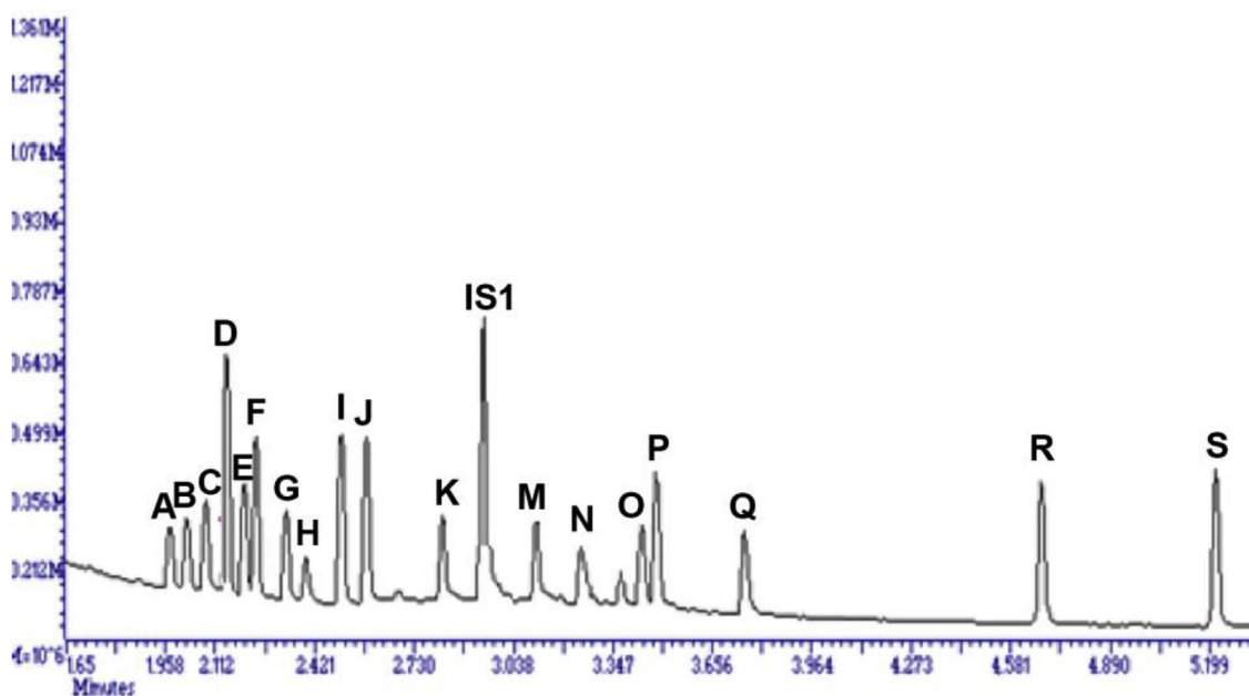
Fig. 2. FAST-GC/MS-TOF analysis of the mixture of 18 synthetic cathinones. A: 4-Fluoromethcathinone (RT: 1.96); B: Methcathinone (RT: 2.02); C: Thiothione (RT: 2.07); D: Dimethylcathinone (RT: 2.15); E: Ethcathinone (RT: 2.21); F: Buphedrone (RT: 2.24); G: 3-Methylmethcathinone (3-MMC) (RT: 2.26); H: Mephedrone (4-MMC) (RT: 2.40); I: 4-Methylmethcathinone (RT: 2.45); J: Pentdrone (RT: 2.51); K: 4-MEC (RT: 2.78); IS1(diphenylamine) (RT: 2.97); M: Brepheдрone (RT: 3.09); N: Methylone (RT: 3.26); O: Ethylone (RT: 3.37); P: Butylone (RT: 3.68); Q: Pentylone (RT: 3.76); R: MDPV (RT: 4.67); S: Naphyrone (RT: 5.21).
