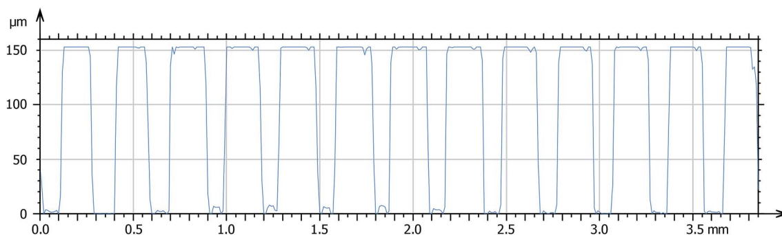
Fig. 7 Lateral profile of printed cylinder from 3KSRD sample with 150 \mu\text{m} in height and diameter.
