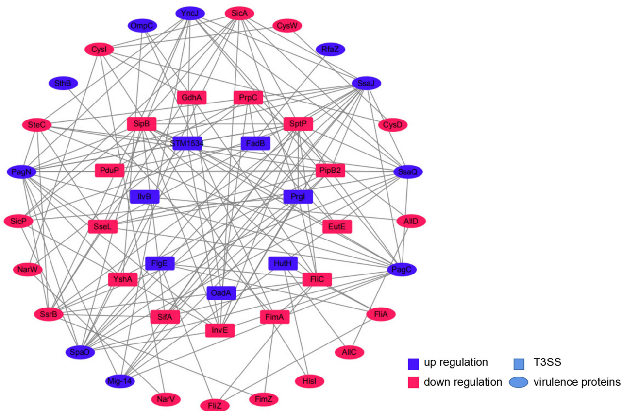
Figure 10 Interaction Network of Differentially Expressed Proteins.
