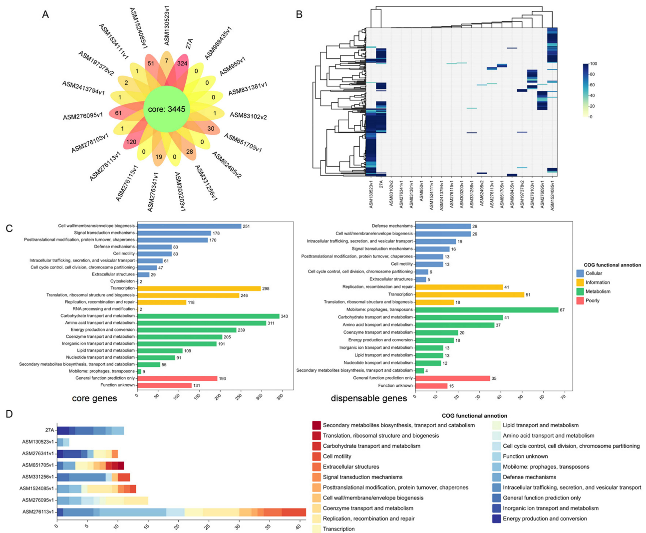
Figure 5 Core and Pan Genes Analysis. (A) Pan genes Venn graph. (B) Core genes and dispensable genes heatmap. (C) COG functional annotation of core genes and dispensable genes. (D) COG functional annotation of specific genes.
