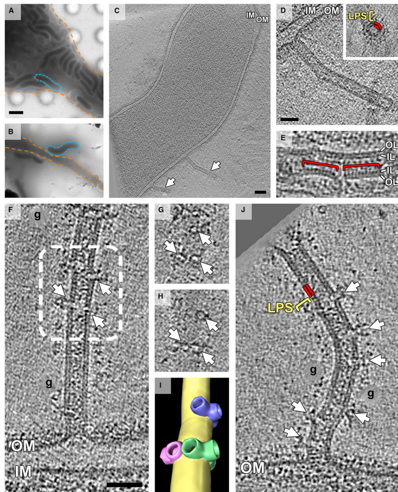
Figure 1. H. pylori Assembles Membranous Tubes When Proximal to Gastric Epithelial Cells (A) Low-magnification view of a gastric epithelial cell grown on an electron microscopy grid and infected with H. pylori . (B) Low-magnification view of H. pylori interacting with a gastric epithelial cell surface. In (A) and (B), blue dashed lines indicate examples of H. pylori that were imaged by ECT, and orange dashed lines demarcate the edges of individual gastric epithelial cells. (C) Tomographic slice through WT H. pylori co-cultured with gastric epithelial cells. Arrows indicate membrane tubes extending from the H. pylori cell envelope. (D) Enlarged view of the longer tube shown in (C). Inset: cross-section of a membrane tube. The two leaflets of the tube membrane bilayer are labeled by two red lines; LPS is indicated by a yellow bracket. (E) Periodic densities lining the inside of the tube (red brackets). (F) An individual tube displaying lateral ports (arrows). (G and H) Distal (G) and proximal (H) cross-sections of ports within the boxed region of the tube depicted in (F). (I) 3D segmentation of the boxed region in (F). (J) Large tomographic slice showing multiple tubes (white arrows) and LPS (yellow bracket).
