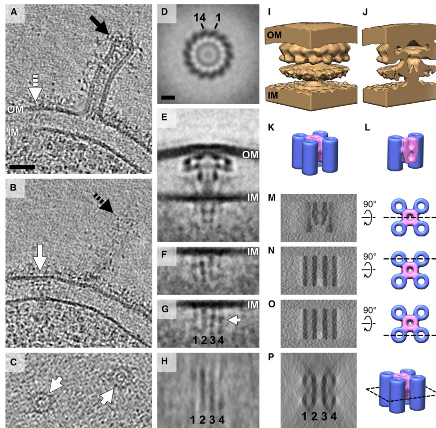
Figure 2. In Vivo Structure of the cag T4SS
