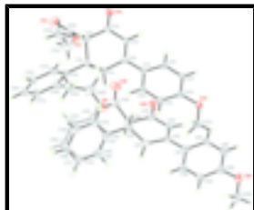
Fig. 1. The asymmetric unit of the title compound, showing 50% probability displacement ellipsoids and the atom-numbering scheme. Both disorder component of an independent molecule are shown.
