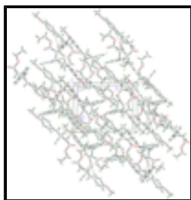
Fig. 2. The crystal packing of the title compound, viewed down the c axis. Only the major disorder component of an independent molecule is shown.
