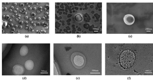
Fig. 8 (a) Is the SEM image of sensor R - \beta -D-1 (5 mg mL -1 in ethanol), (b) is the SEM image of R - \beta -D-1 with Fe 3+ , (c) is the SEM image of L-Cys added to R - \beta -D-1-Fe 3+ , (d) is the TEM image of sensor R - \beta -D-1, (e) is the TEM image of Fe 3+ added to sensor R - \beta -D-1; (f) is the TEM plot of the addition of L-Cys in R - \beta -D-1-Fe 3+ .
