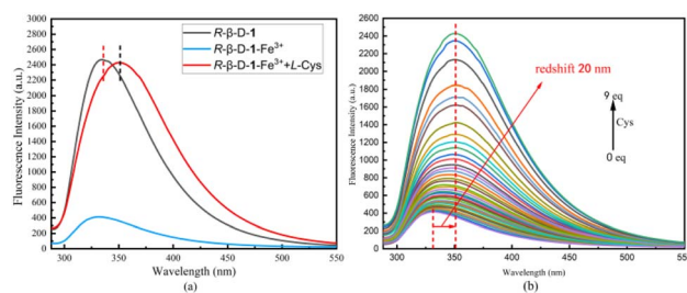
Fig. 6 (a) Is a fluorescence control plot of R\text{-}\beta\text{-D-1} , R\text{-}\beta\text{-D-1} + 10 \text{ eq. Fe}^{3+} , R\text{-}\beta\text{-D-1} + 10 \text{ eq. Fe}^{3+} + 10 \text{ eq. L-Cys} , with the remaining amino acids identified in the ESI.† (b) Fluorescence titration plot of R\text{-}\beta\text{-D-1-Fe}^{3+} ( 20 \mu\text{M} in MeOH, 10 \text{ eq. Fe}^{3+} , \lambda_{\text{ex}} = 278 \text{ nm} ) with gradual increase in Cys ( 0.01 \text{ M} ) equivalents ( 0\text{-}9 \text{ eq.} ).
