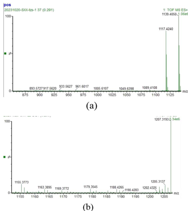
Fig. 5 (a) ESI-MS variation of R\text{-}\beta\text{-D-1} ; (b) ESI-MS variation of R\text{-}\beta\text{-D-1-Fe}^{3+} .
