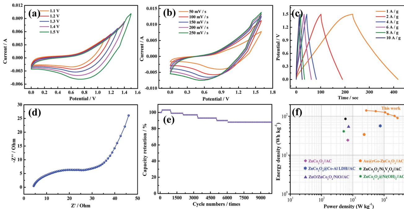
Fig. 5 Electrochemical characterizations of the ASC (a) CV curves of the \text{ZnCo}_2\text{O}_4@PPy//AC ASC at different voltage windows (b) CV curves of the \text{ZnCo}_2\text{O}_4@PPy//AC ASC at different scan rates (c) GCD curves (d) Nyquist plots (e) cycling performance (f) Ragone plots.
