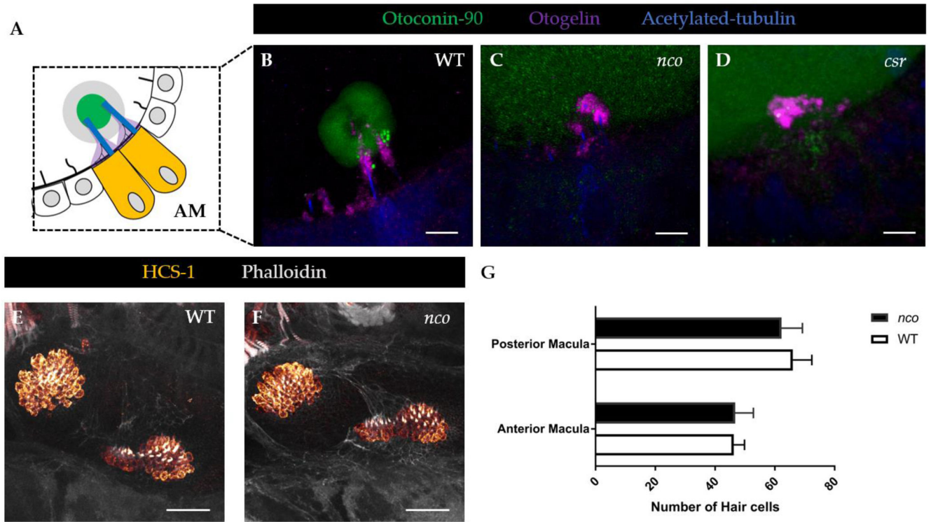
Figure 5: Aberrant expression of proteins involved in otolith development in csr and nco . (A) Schematic of anterior macula (AM) tethered to otolith at 27 hpf. (B) In WT, Otoconin-90 (Oc90) is expressed within the mineralized otolith, which is situated atop the otolithic membrane (Otogelin, or Otog), at 27 hpf. Scale bar = 5 \mu m. (C-D) Oc90 has diffuse expression within the otocyst of csr and nco . In csr and nco , Otog is localized near the apical surface of hair cells. (E-F) Expression showing hair cells in WT and nco larvae at 5 dpf. Scale bar = 25 \mu m. (G) Quantification of hair cell numbers in the posterior and anterior macula of WT and nco (n = 4).
