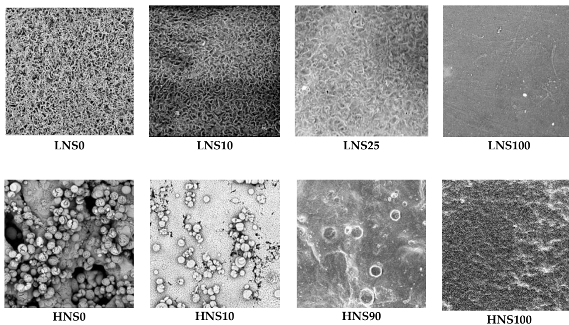
Figure 1. Selected scanning electron microscopy (SEM) images of (top) nylon610-silk (LNS) blend films and (bottom) nylon1010-silk (HNS) blend films. (each image scale is 150 \mu\text{m} \times 150 \mu\text{m} ).
