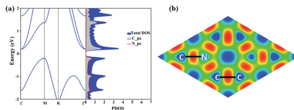
Fig. 2 (a) Electronic band structure and projected density of state (PDOS). \Gamma (0.0, 0.0, 0.0), M ( 1/2 , 0.0, 0.0) and K ( -1/3 , 2/3 , 0.0) refer to special points in the first Brillouin zone. (b) The electron localisation function (ELF) of C_3N .
