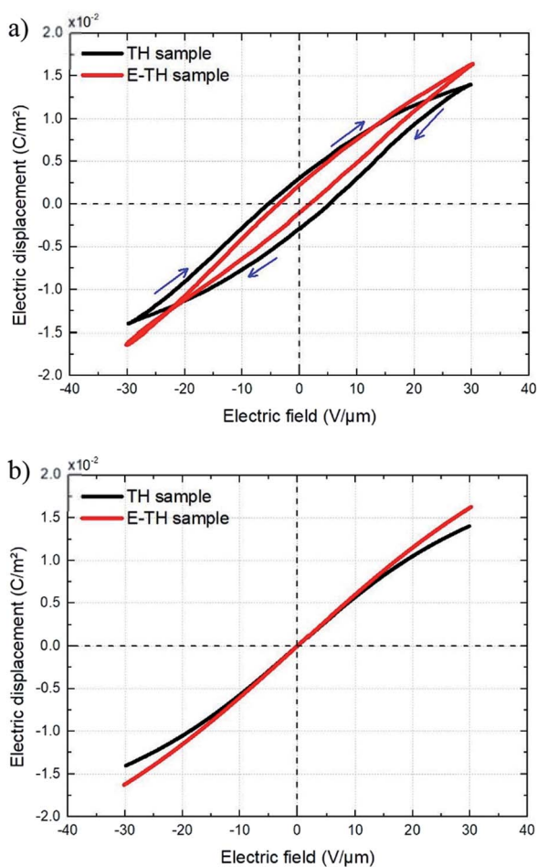
Fig. 12 (a) Superposition of experimental electric displacement curves and (b) modeled polarization for the two samples. Direction of applied electric field is indicated by blue arrows.
