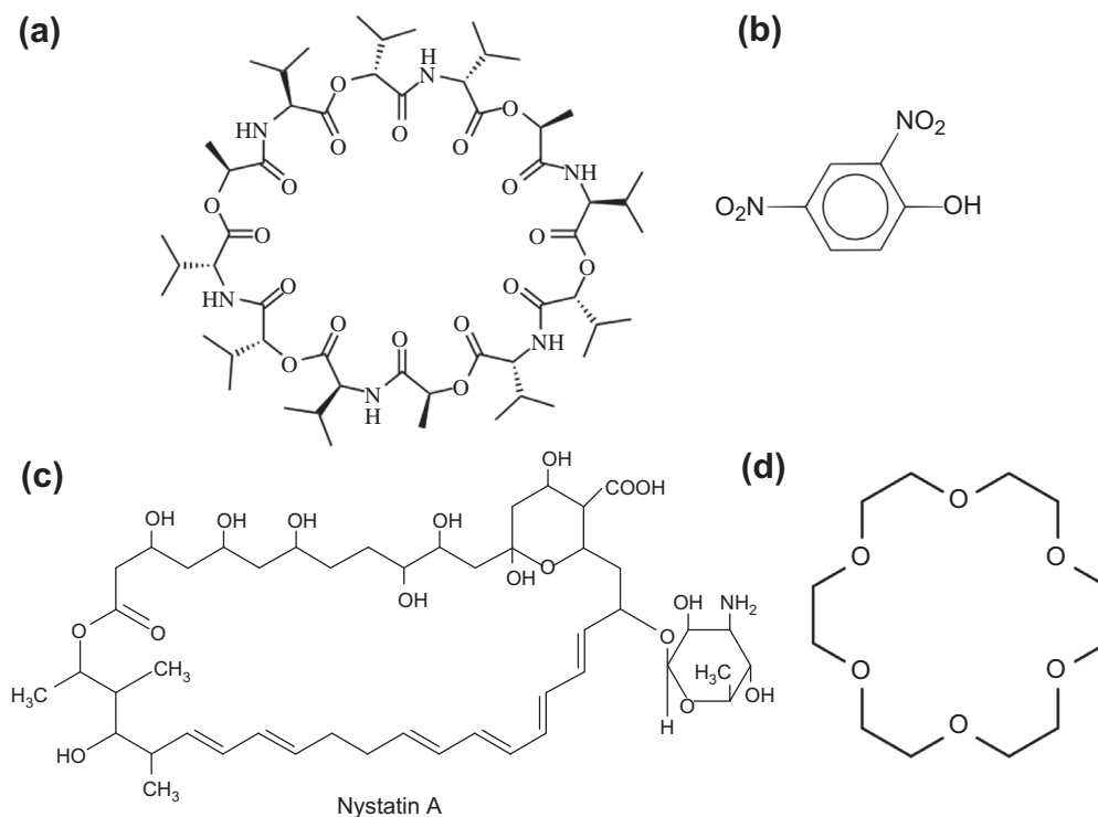
FIGURE 14.19 Representative examples of ionophores: (a) Valinomycin (b) 2,4-dinitrophenol (c) Nystatin (d) Crown ether.
