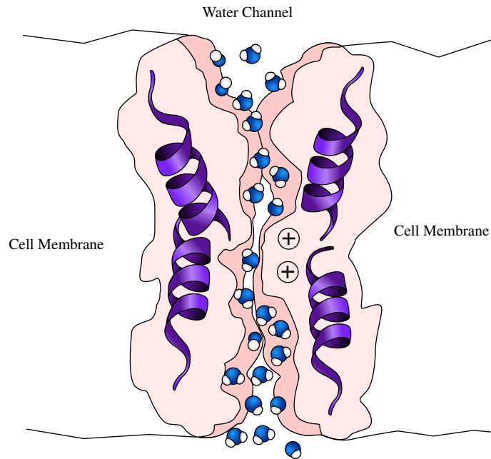
FIGURE 14.12 Aquaporin [17]. Water molecules pass through the aquaporin channel in single file.
