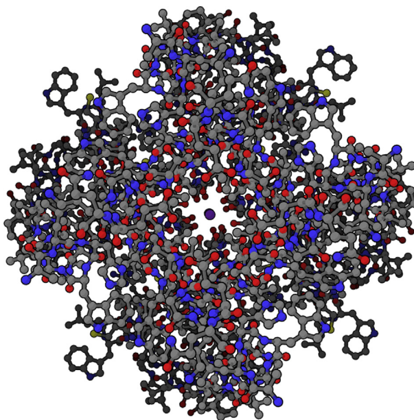
FIGURE 14.7 Three-dimensional structure of the potassium channel [12]. The channel itself is the clear opening in the center of the structure and a single K^+ is shown in the center of the channel.
