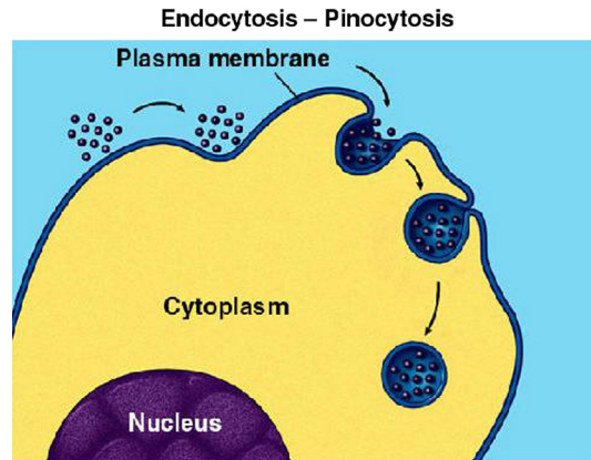
FIGURE 14.24 Pinocytosis, a type of endocytosis. An invagination of the plasma membrane encapsulates many water-soluble solutes ranging in size from salts to macromolecules. Courtesy of Dr. Gary Kaiser
