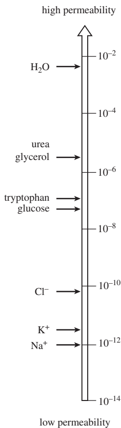
FIGURE 14.1 Log of the permeability ( P in cm/s) across lipid bilayer membranes for common solutes ranging from \text{Na}^+ ( 10^{-12} \text{ cm/s} ) to water ( 0.2 \times 10^{-2} \text{ cm/s} ). This range spans almost 10 orders of magnitude [1].
