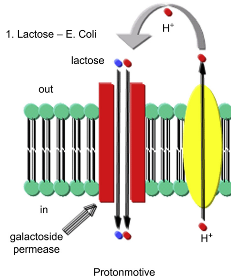
FIGURE 14.16 Lactose transport system in Escheria coli [21]. Uptake of lactose is coupled to the movement of \text{H}^+ down its electrochemical gradient. This is an example of active transport, co-transport, and active symport.
