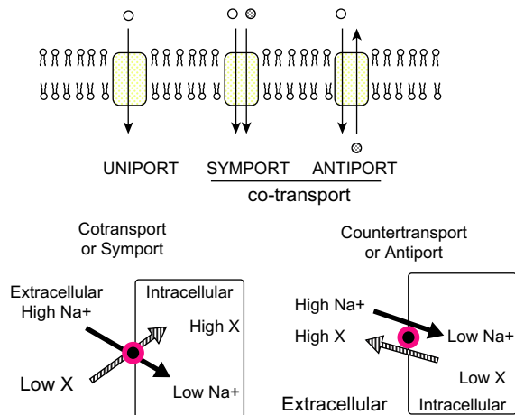
FIGURE 14.13 Basic types of active transport [18].
