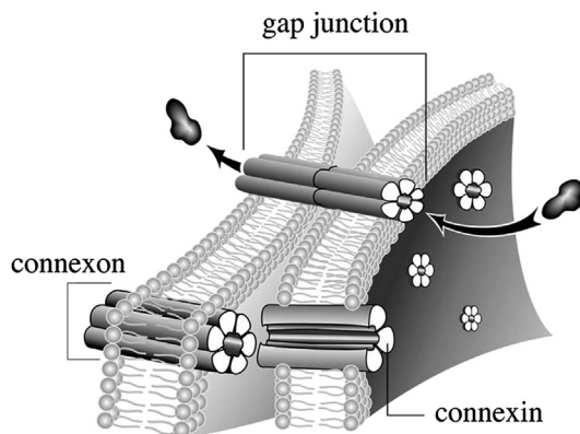
FIGURE 14.21 Gap junction [43]. Six connexins form a connexon and one connexon from each cell unite to form a gap junction.
