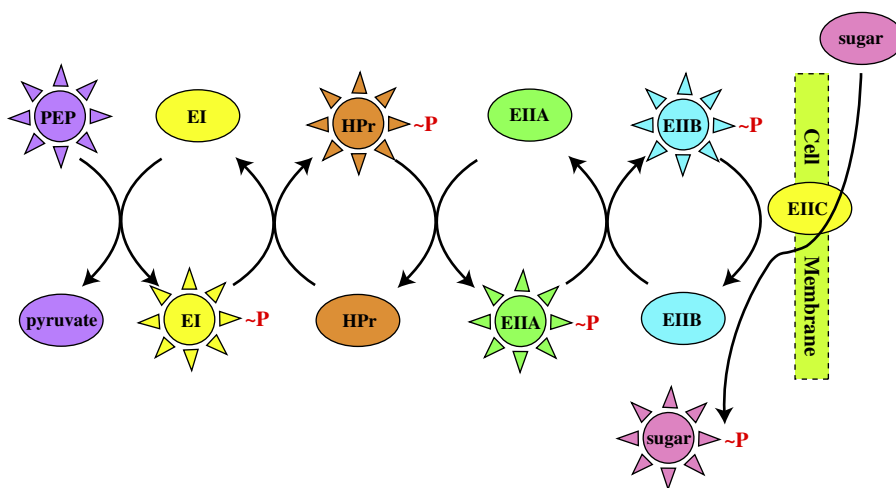
FIGURE 14.17 The bacterial PTS system for glucose transport [27].
