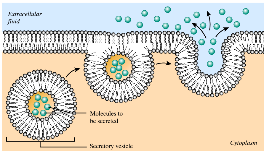
FIGURE 14.26 Exocytosis. Intra-cellular secretory vesicles fuse with the plasma membrane releasing their water-soluble contents to the outside and adding membrane material to the plasma membrane [56].
