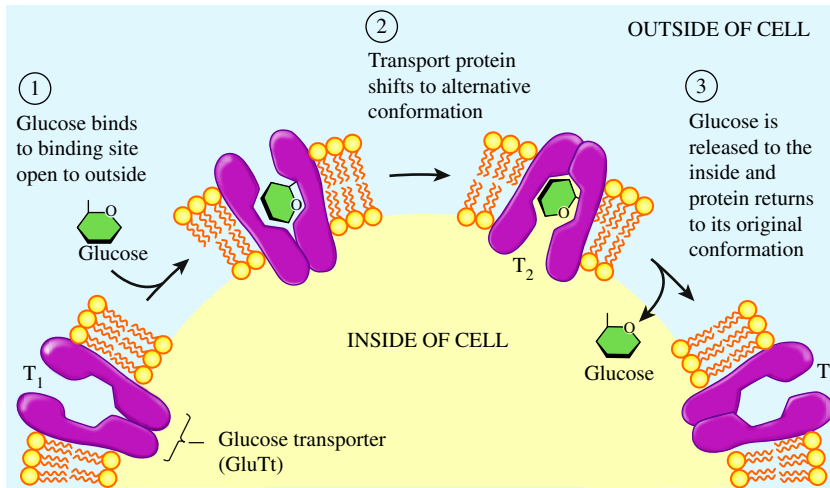
FIGURE 14.6 Glucose facilitated diffusion transporter GLUT-1 [10].
