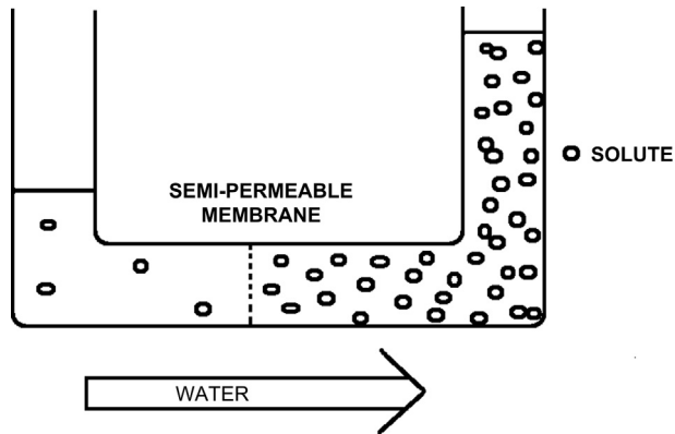
FIGURE 14.3 Osmosis and osmotic pressure. Water is placed in a U-shaped tube where each of the tube arms is separated by a semi-permeable membrane with pores of a size that water can easily pass through but a solute cannot. Upon addition of the solute to the tube's right arm, water diffuses from left to right (high water potential to low). The column of water in the tube's right arm (the one containing the solute) rises until the extra weight of the column equals the osmotic pressure caused by the solute. A pump could then be used to counter the osmotic pressure whereupon the solution columns in the right and left arms of the tube are made the same. The pump pressure required to equalize the height of the two columns is the osmotic pressure [4]. Note a small amount of solute leaks from right to left since no filter is perfect.
