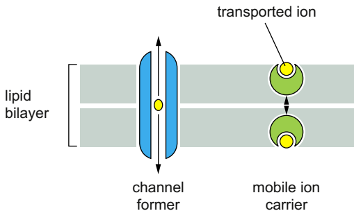
FIGURE 14.18 Two basic types of ionophores, channel formers (left) and mobile carriers (right) [30].
