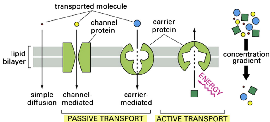
FIGURE 14.4 Basic types of membrane transport: simple passive diffusion; facilitated diffusion (by channels and carriers); and active transport [8].
