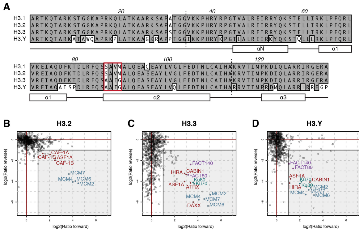
Figure 1. Identification of human H3 variant chaperone complexes. (A) Amino acid alignment of human H3.1, H3.2, H3.3 and H3.Y proteins using ClustalW Alignment (MacVector 13.5.1). Identical amino acids are depicted in dark gray, similar amino acids in light gray and differences are highlighted with a white background. N- and C-terminal tails are separated by dotted lines and a schematic representation of the secondary structures is shown below the alignment. The known chaperone recognition sites of H3.1, H3.2 and H3.3 are boxed. (B–D) eGFP-pull-downs for H3 variant-specific chaperone complexes are shown. HK cells stably expressing eGFP-H3.2 (B), eGFP-H3.3 (C) and eGFP-H3.Y (D) were SILAC labeled and subjected to single-step affinity purification of soluble nuclear proteins using GFP nanotrap beads. In each panel, the ratio between pull-down of the transfected cell line and a control cell line for all identified proteins after MS is plotted. Proteins known to interact with H3 variants are indicated. Background binders and potential contaminants are shown as black dots and are listed together with all identified proteins in Supplementary Tables S1–3.
