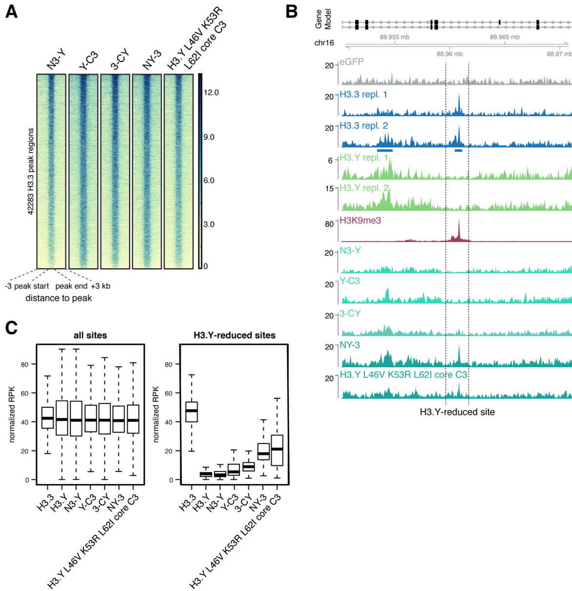
Figure 7. Restoration of DAXX binding to H3.Y mutants enables deposition at heterochromatin sites. (A) ChIP-seq density heat map of H3.3 as described in Figure 3C listing H3.3/H3.Y ‘tail-swap’ and H3.Y L46V K53R L62I core C3 mutant signals. Data for H3K9me3 is from (64) (GEO repository sample GSM2308949 (GSE86811)). Color intensity represents normalized and globally scaled tag counts. (B) Genome browser snap shot of representative region displaying ‘tail-swap’ and H3.Y L46V K53R L62I core C3 mutant signals (turquoise) ChIP-seq signals at H3.3-enriched, H3.Y-reduced heterochromatin sites (see Figure 3D). (C) Box plot of peak signal intensities of H3.3/H3.Y ‘tail-swap’ and H3.Y L46V K53R L62I core C3 mutant signals comparing all H3.3-enriched sites with H3.Y-reduced sites. Shown are mean signal intensities of two H3.3 and H3.Y replicates. Testing for statistical significance of observed differences was done using Wilcoxon-signed-rank test (Supplementary Table S10).
