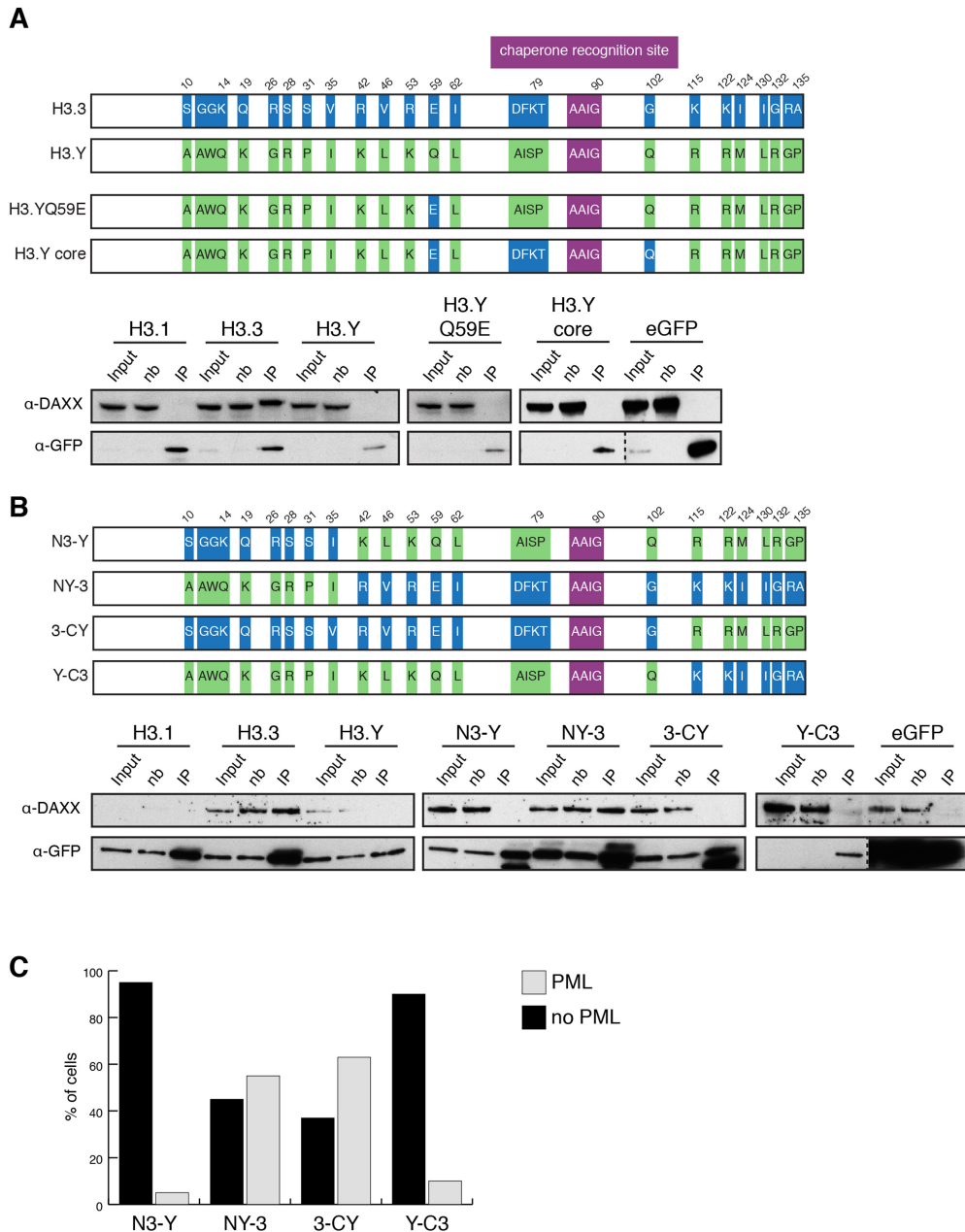
Figure 5. H3.3 core region in combination with C-terminal sequence is sufficient for DAXX interaction. (A and B) Top: schematic alignment of H3.3, H3.Y and H3.Y core (A) and H3.3/H3.Y ‘tail-swap’ (B) mutant proteins. H3.3-specific amino acids are highlighted in blue, whereas H3.Y-unique residues are depicted in green boxes. Shared chaperone recognition sequence is shown in purple. Bottom: soluble nuclear extracts from HK cells stably expressing eGFP-tagged H3 variants as well as H3.YQ59E and H3.Y core (A) or H3.Y/H3.3 ‘tail-swap’ mutants (B) were used for pull-down experiments as described in Figure 2A. One out of at least two representative immunoblots is shown. Proper nuclear and chromatin localization of all eGFP-H3 variants and H3.Y core mutants is shown in Supplementary Figures S3 and 4 and of chimeric constructs in Supplementary Figure S5A and B. (C) Quantification of 200 cells 24 h after transfection (see Supplementary Figure S5C for IF analysis) showing the localization of different eGFP-H3.3/H3.Y ‘tail-swap’ mutants to PML-NBs (gray) or not (black).
