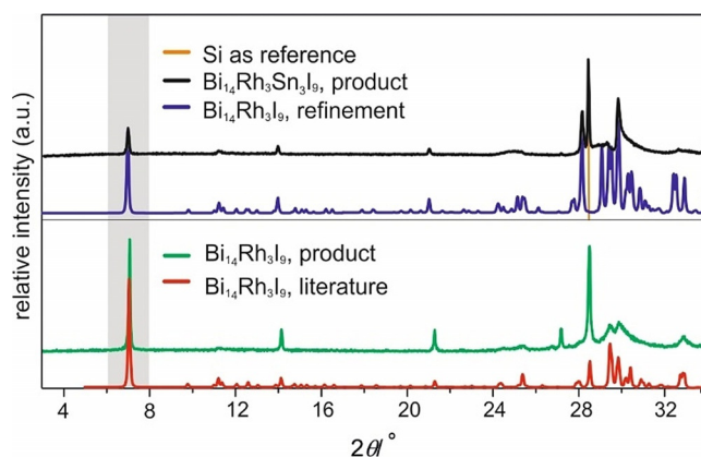
Figure 3. PXRD pattern (Cu K_{\alpha 1} , top) of the product of a mixture of Bi, Rh, Sn, and BiI 3 (12:3:3:9) reacted at 310 °C (black), compared to the theoretical pattern (red) and measured pattern (green) of Bi 14 Rh 3 I 9 , as well as the refined pattern with TOPAS (blue).
