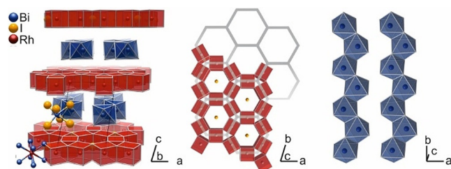
Figure 1. (left) Crystal structure of \text{Bi}_{14}\text{Rh}_3\text{I}_9 (colour code: bismuth = blue, rhodium = red, iodine = orange); (middle) 2D TI layer \infty^2[(\text{Bi}_4\text{Rh})_3\text{I}]^{2+} : edge-sharing [\text{Bi}_4\text{Rh}] cubes forming a hexagonal shaped network with iodine atoms in the hexagonal prismatic voids (red-coloured polyhedra); (right) topologically trivial spacer \infty^1[\text{Bi}_2\text{I}_6]^{2-} : parallel iodido-bismuthate chains of edge-sharing octahedra (blue-coloured polyhedra).
