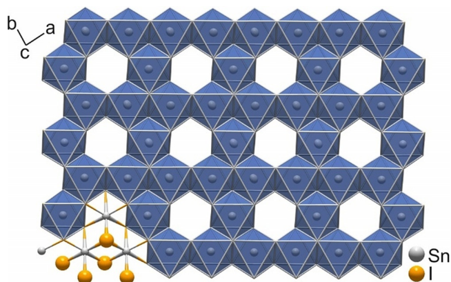
Figure 6. Anionic spacer layer \infty^2[\text{Sn}_3\text{I}_6]^{2-} in \text{Bi}_{12}\text{Rh}_3\text{Sn}_3\text{I}_9 with tin(II) cations forming a [3.6.3.6; 3^2.6^2 ] net.
