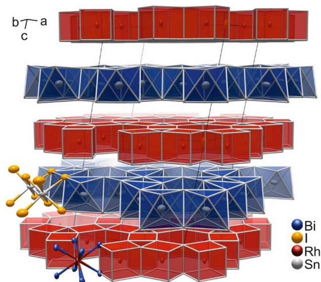
Figure 5. Crystal structure of Bi 12 Rh 3 Sn 3 I 9 . The intermetallic kagome network \infty^2[(\text{Bi}_4\text{Rh})_3\text{I}]^{2+} (red) alternates with the anionic spacer layer \infty^2[\text{Sn}_3\text{I}_8]^{2-} (blue).
