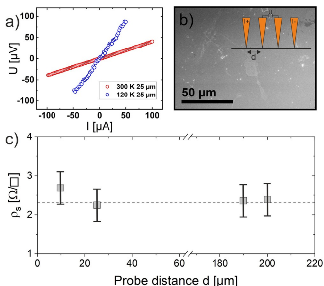
Figure 9. Resistivity of \text{Bi}_{12}\text{Rh}_3\text{Sn}_3\text{I}_9 measured by in situ four-point probe technique. a) U curves for fixed probe spacing at 120 and 300 K. b) SEM image of \text{Bi}_{12}\text{Rh}_3\text{Sn}_3\text{I}_9 . The inset shows the collinear four-point probe geometry. c) Averaged resistivity as a function of probe distance d measured at 300 K.
