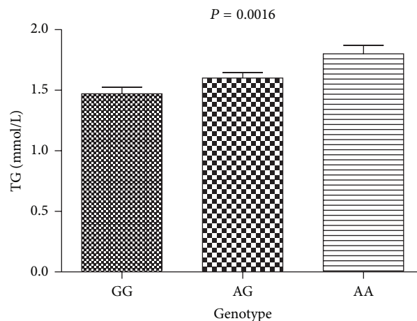
FIGURE 2: Association between TG concentrations and GCKR rs780093 polymorphism. TG concentrations are expressed as mean \pm SEM.
