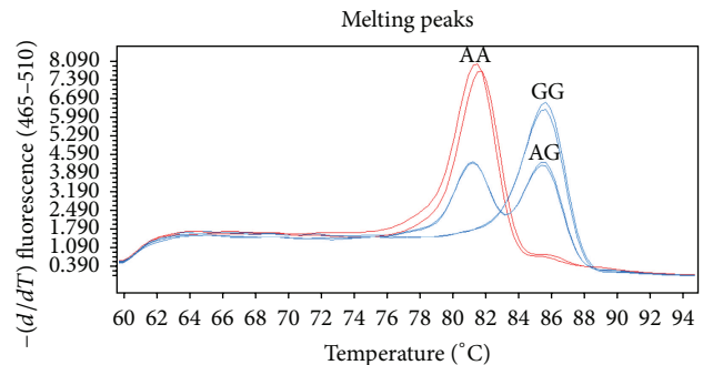
FIGURE 1: Genotyping of GCKR rs780093 using T m -shift method. GG genotype has higher T m value, namely, the 5' end to join long sequences of alleles homozygous. AA genotype has lower T m value, namely, the 5' end to join short sequences of alleles homozygous. AG has the mixed curves with low and high T m values.
