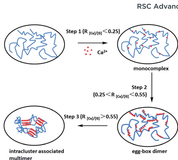
Fig. 1 Schematic drawing of the multiple-step binding of \text{Ca}^{2+} to alginate with a considerable chain length. The zigzag lines, smooth lines, and dots stand for G-block, M-block, and \text{Ca}^{2+} , respectively. R_{[\text{Ca}]/[\text{G}]} is the feeding ratio of added \text{Ca}^{2+} to unit G residue. This figure has been adapted from ref. 50 with permission from American Chemical Society, Copyright © 2007.
