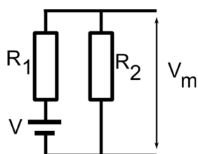
Figure 5. The electrical model for a membrane containing lysenin channels in both open and sub-conducting states. The model includes a voltage source V , open channels of total resistance R_1 , and sub-conducting channels of total resistance R_2 . The resulting membrane voltage V_m may be estimated from the electrical parameters of the equivalent circuit.
