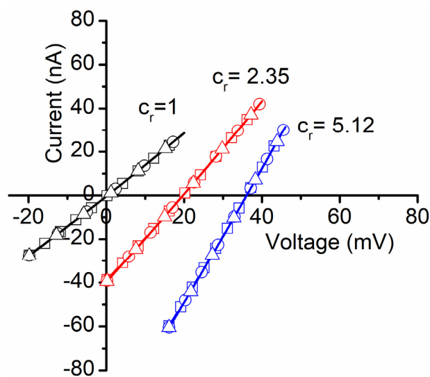
Figure 1. Experimental determination of membrane voltages for lysenin channels reconstituted into planar BLMs. The addition of NaCl to the grounded reservoirs leads to a right shift of the IV plots, indicative of membrane voltage occurrence. An individual experiment employed three IV sweeps for each NaCl concentration ratio c_r , and their average was used to calculate the membrane voltage as the x-intercept. All the points in the plots are experimental; the symbols have been added as visual aids to discriminate between sweeps recorded in identical experimental conditions.
