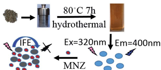
Fig. 1 Schematic illustration of the synthesis process of CDs and detection of MNZ via IFE.
